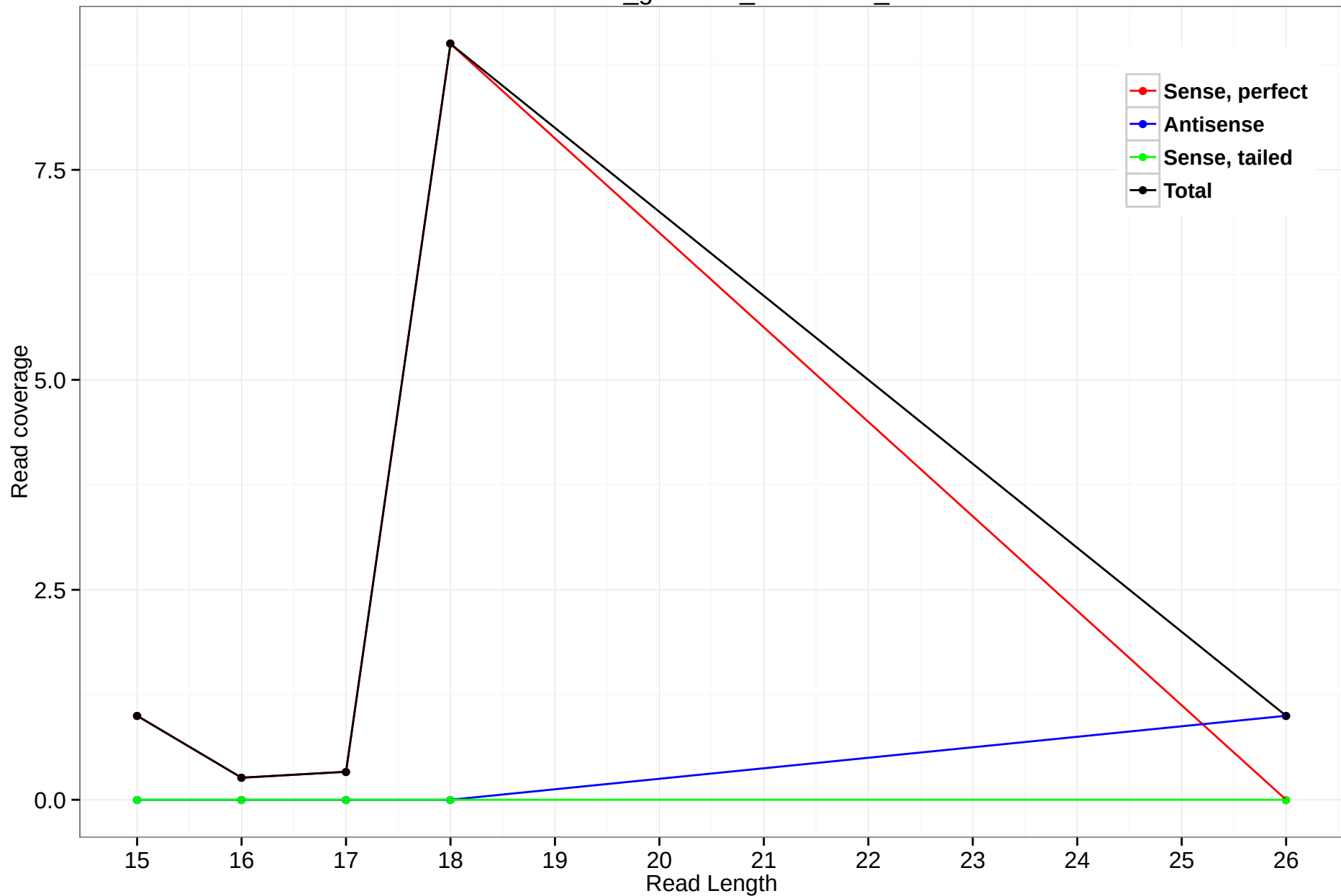
rheMac3_genscan_chr5.1132_6
