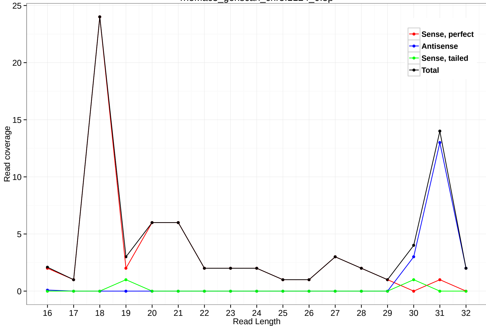
rheMac3_genscan_chr5.1124_0.5p
