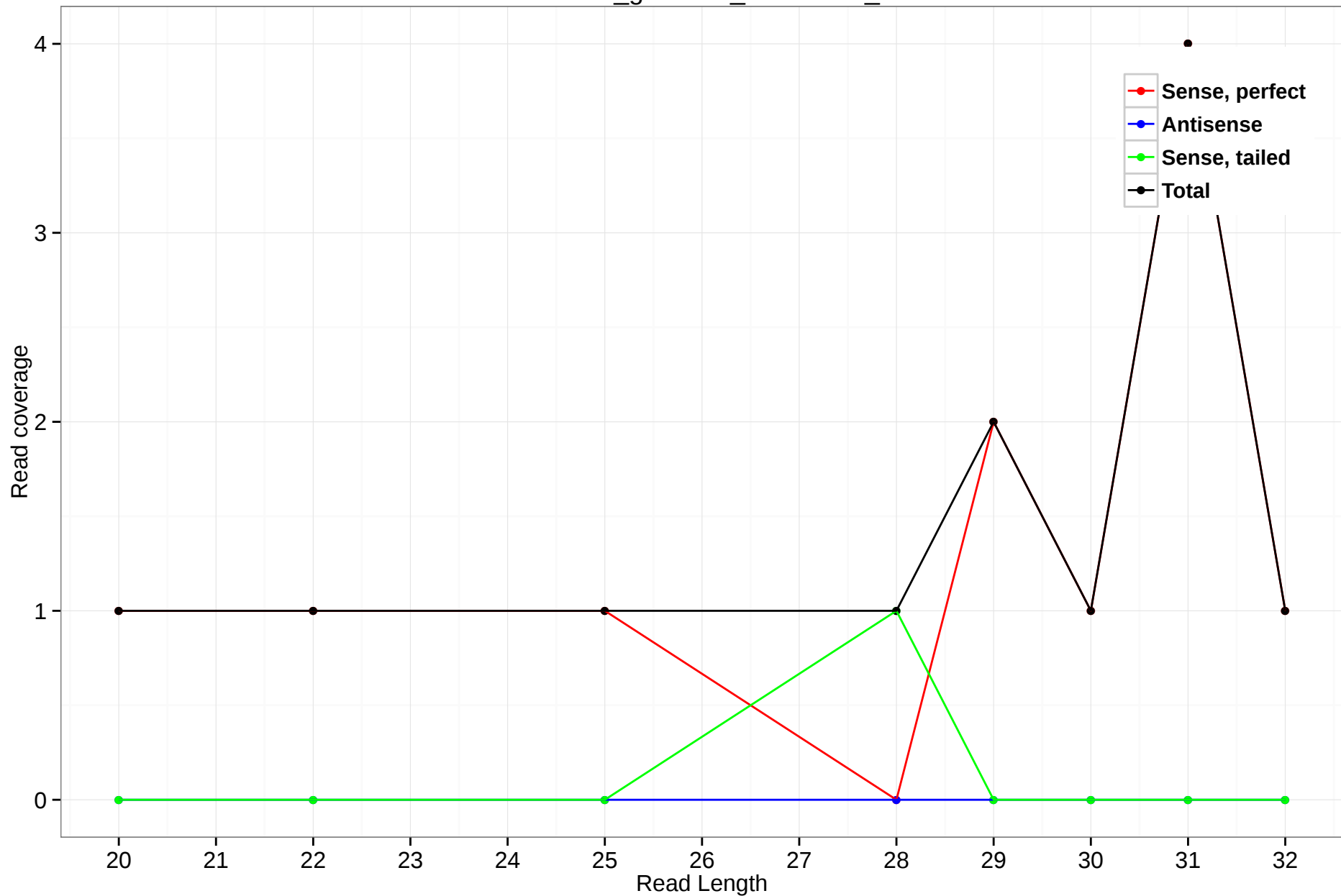
rheMac3_genscan_chr5.1021_2
