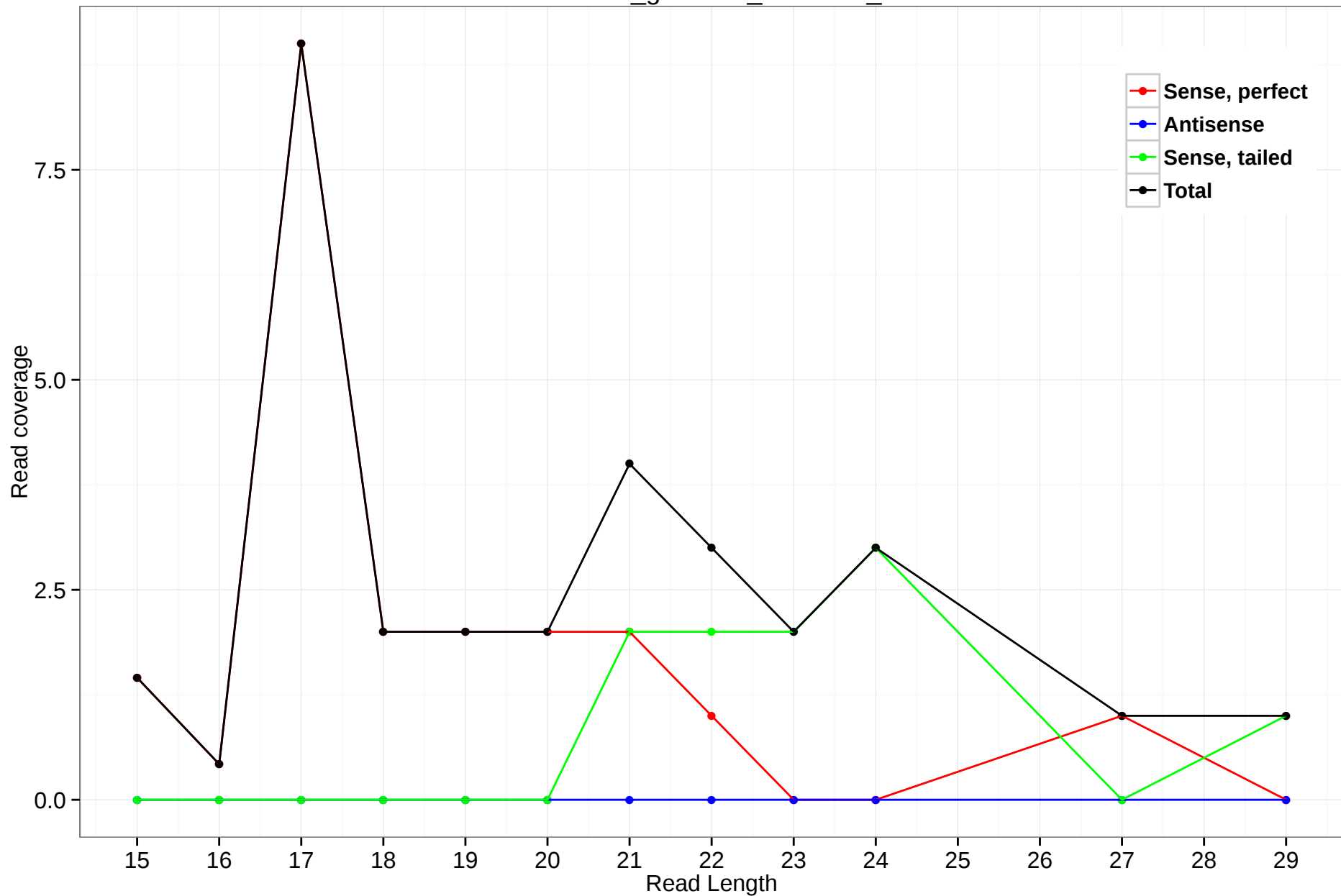
rheMac3_genscan_chr4.992_5
