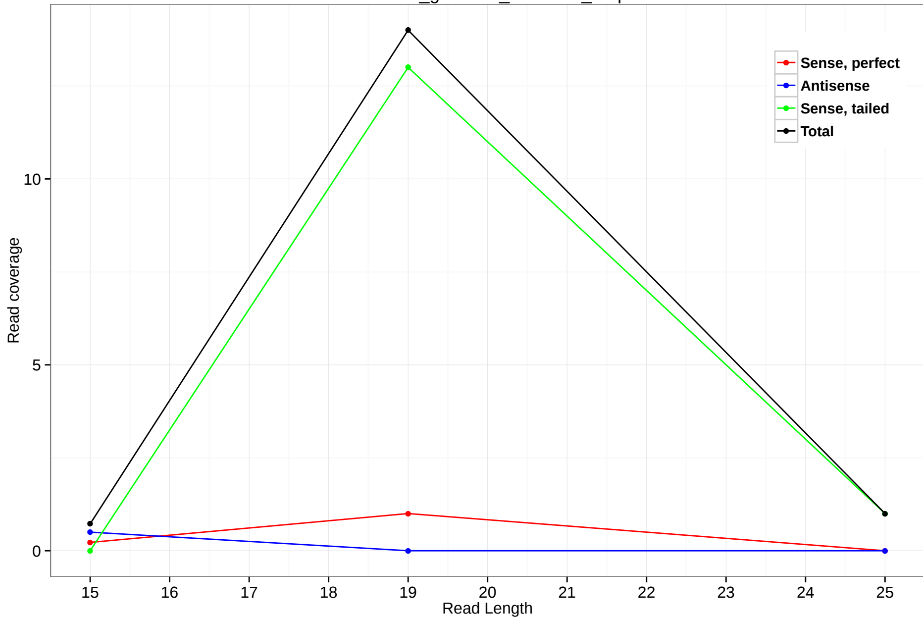
rheMac3_genscan_chr4.989_7.3p
