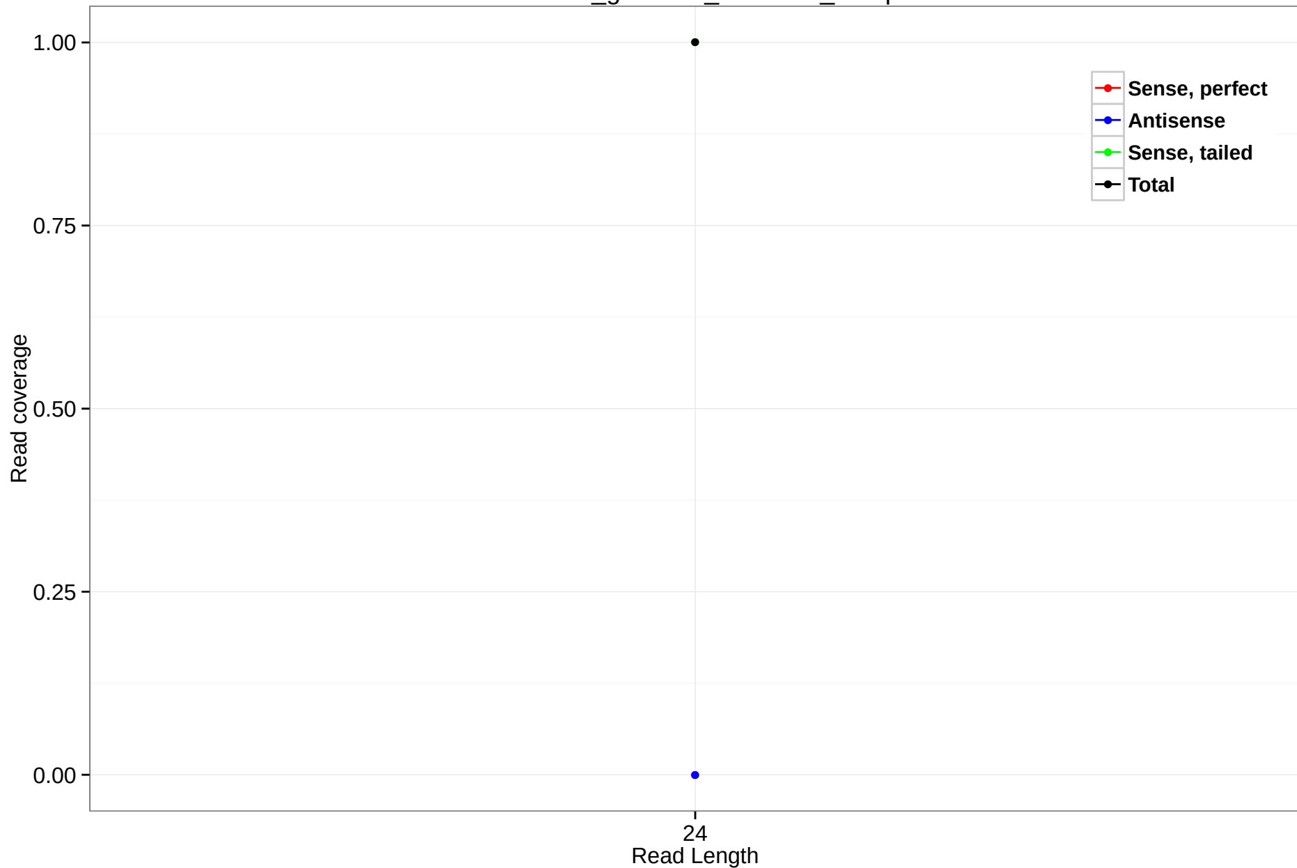
rheMac3_genscan_chr4.986_10.3p
