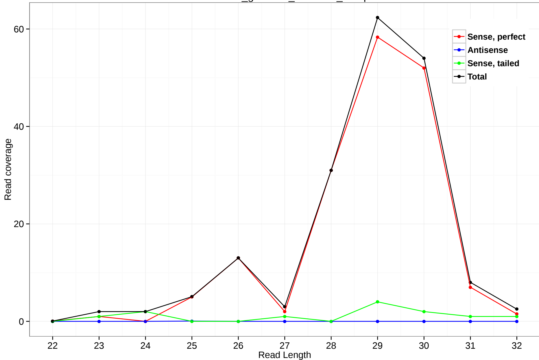
rheMac3_genscan_chr4.985_30.3p
