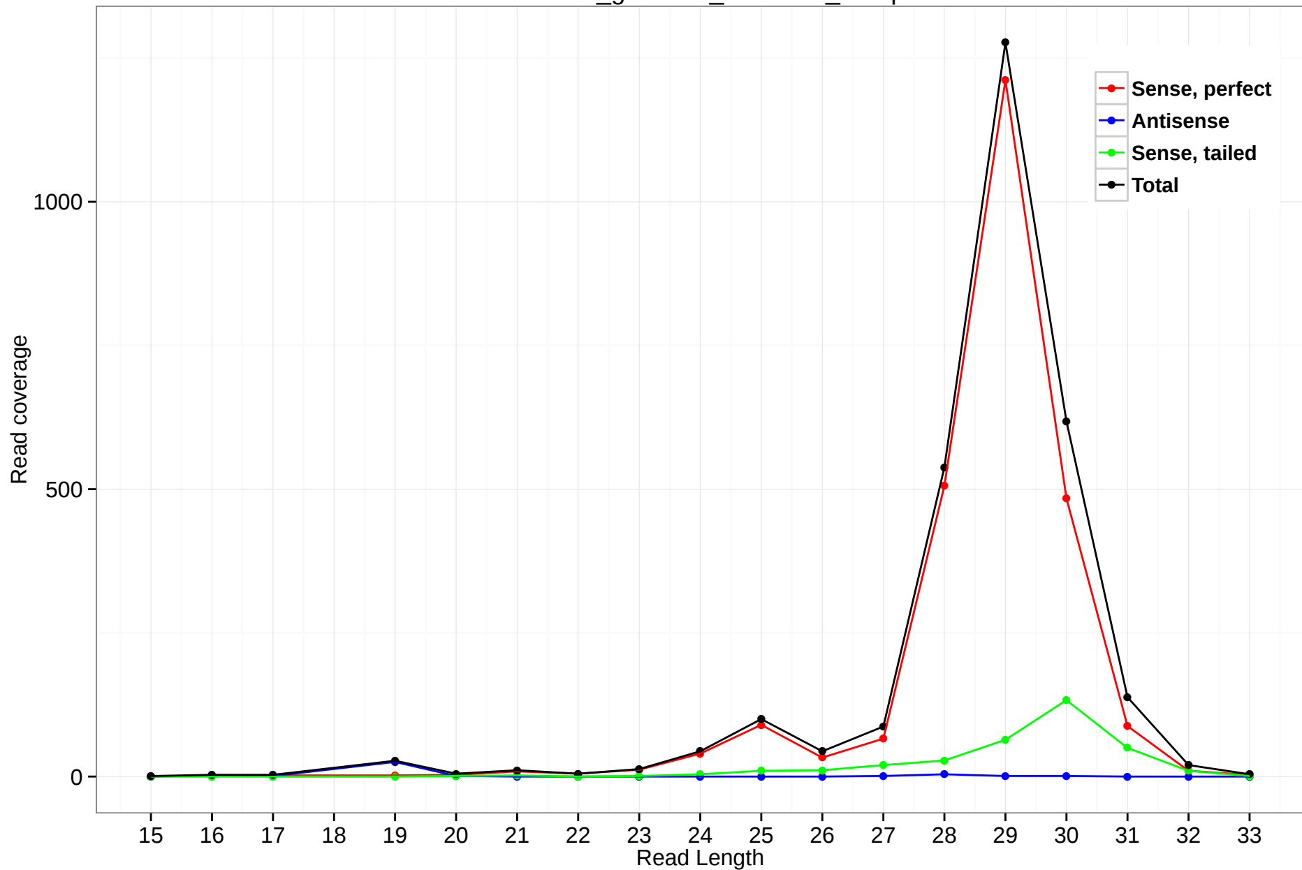
rheMac3_genscan_chr4.985_29.5p
