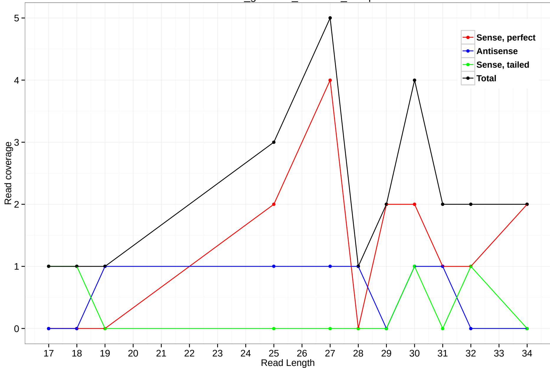
rheMac3_genscan_chr4.984_10.5p
