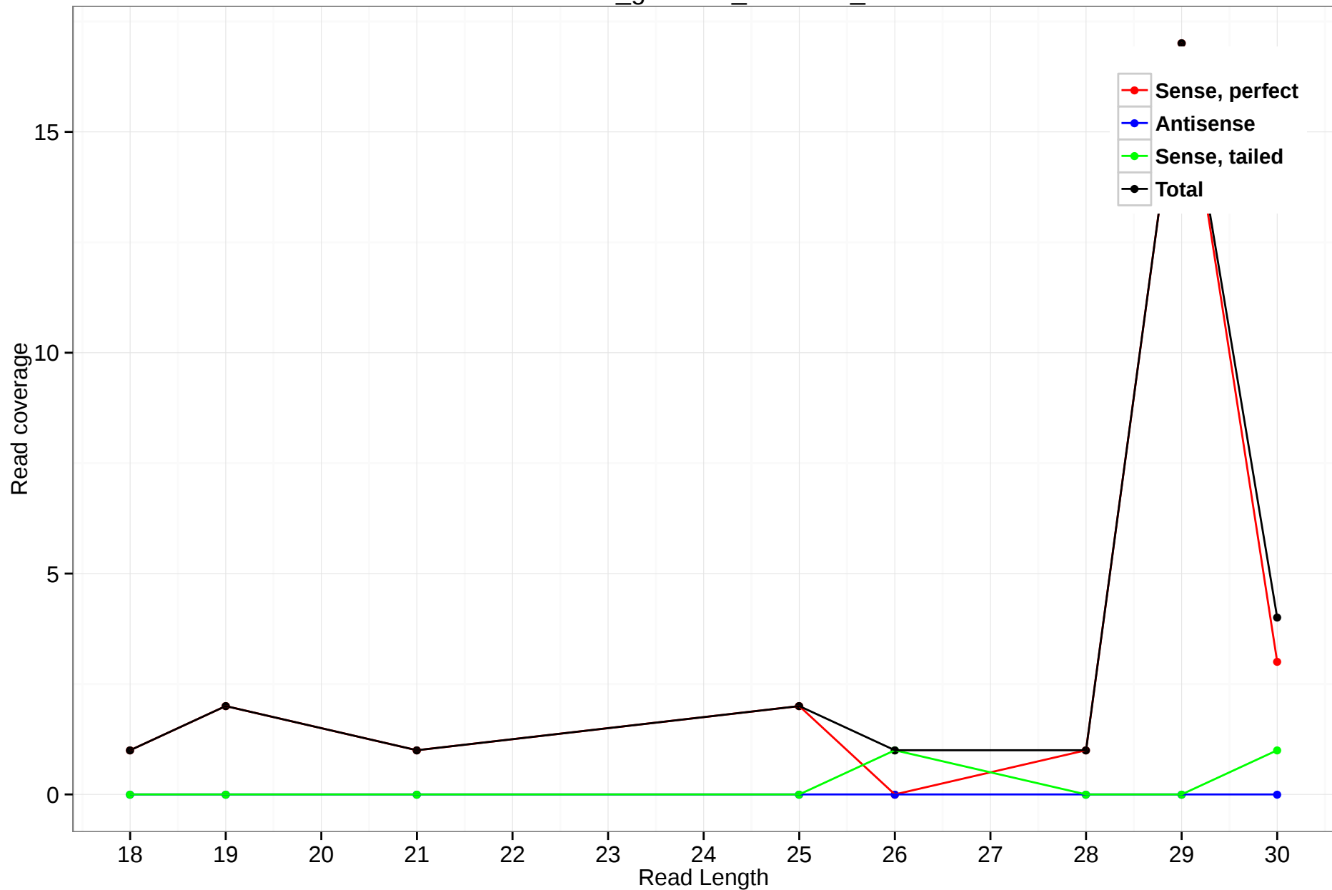
rheMac3_genscan_chr4.964_13
