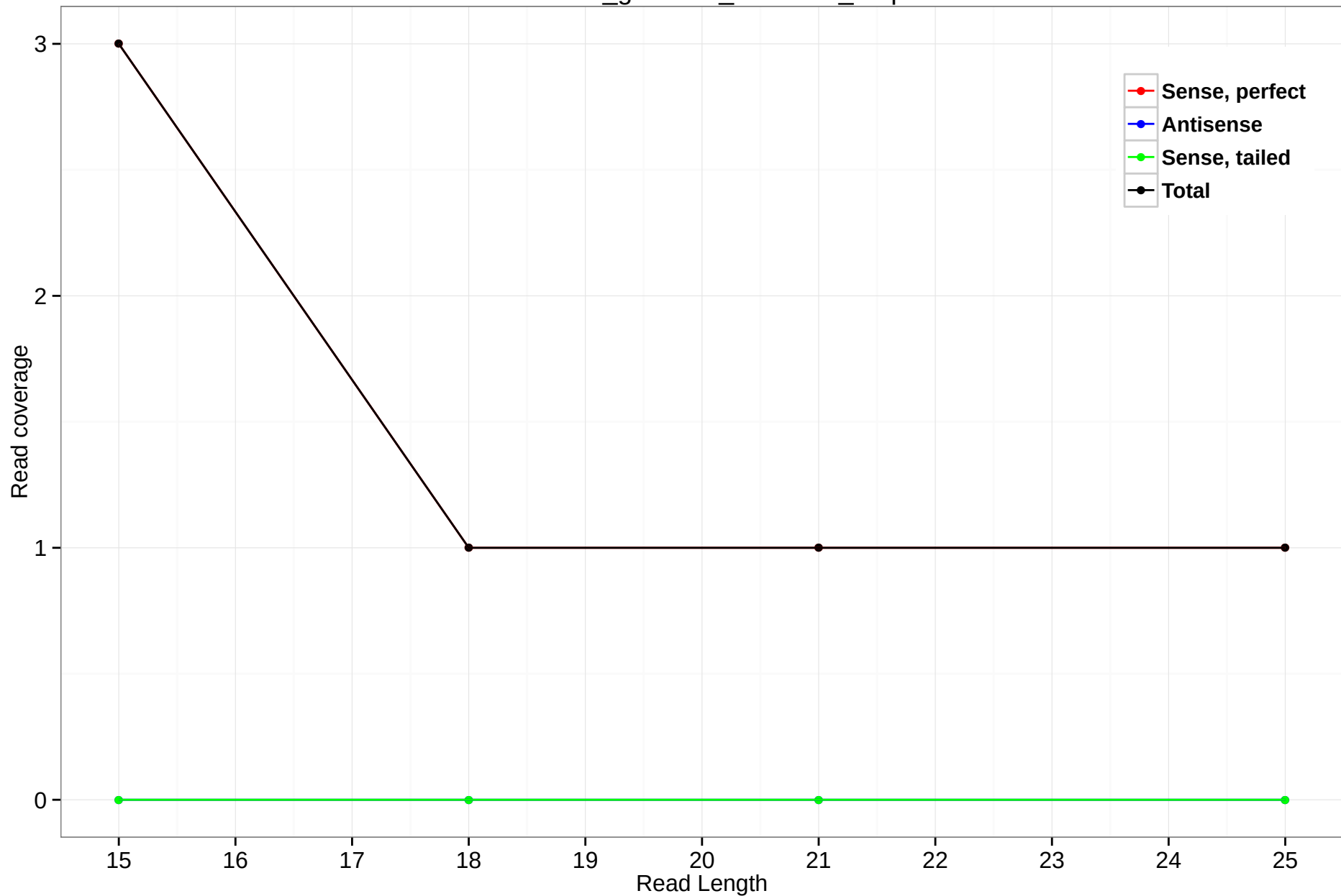
rheMac3_genscan_chr4.964_0.5p
