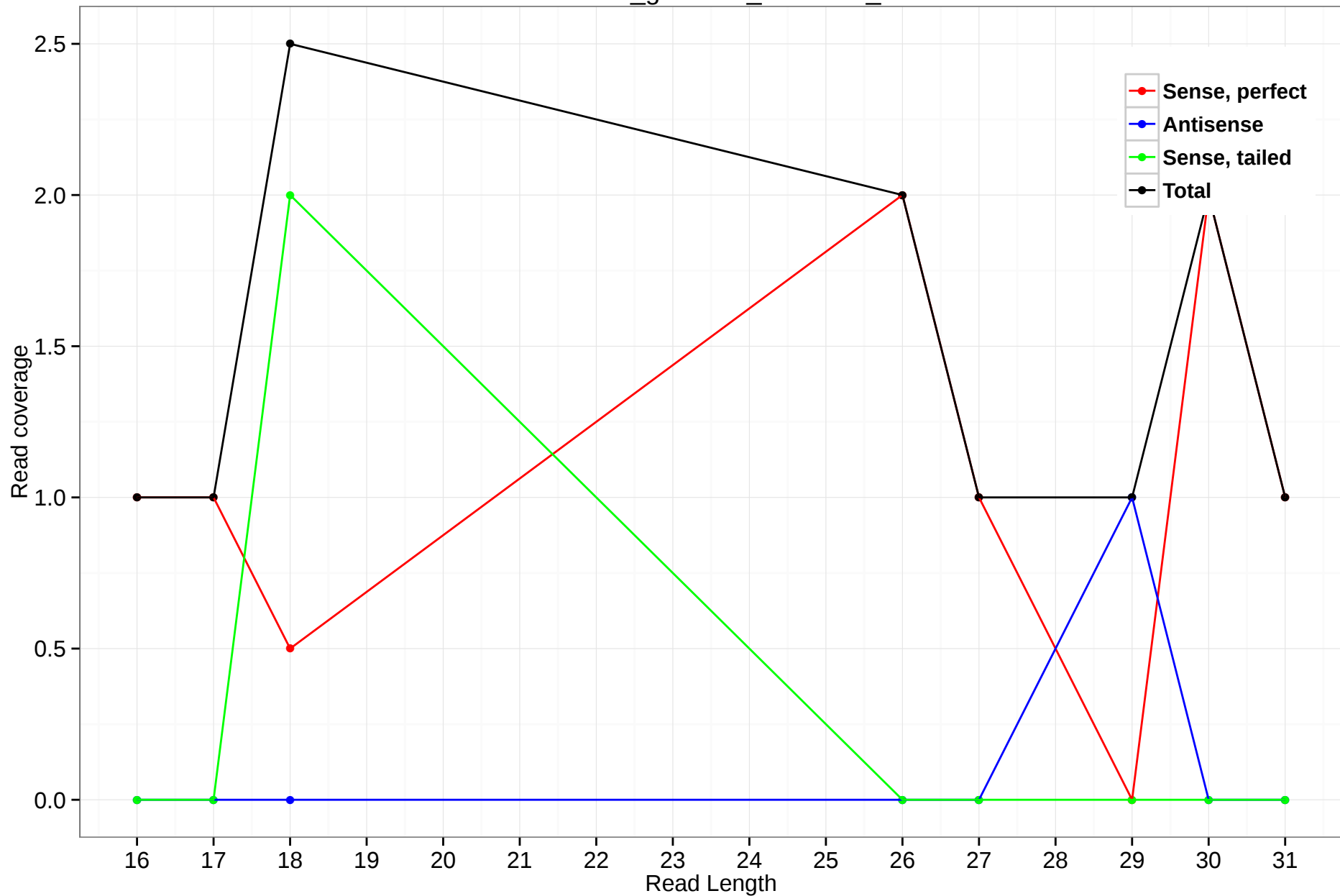
rheMac3_genscan_chr4.959_0
