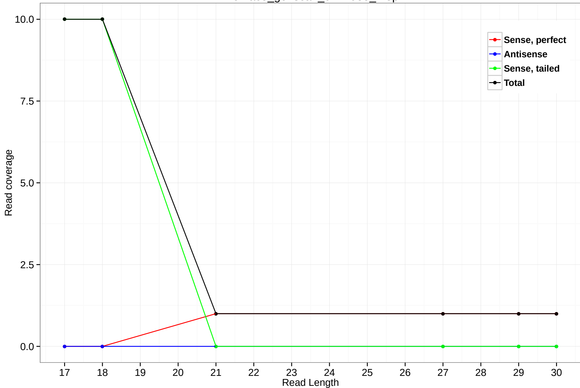
rheMac3_genscan_chr4.955_1.5p
