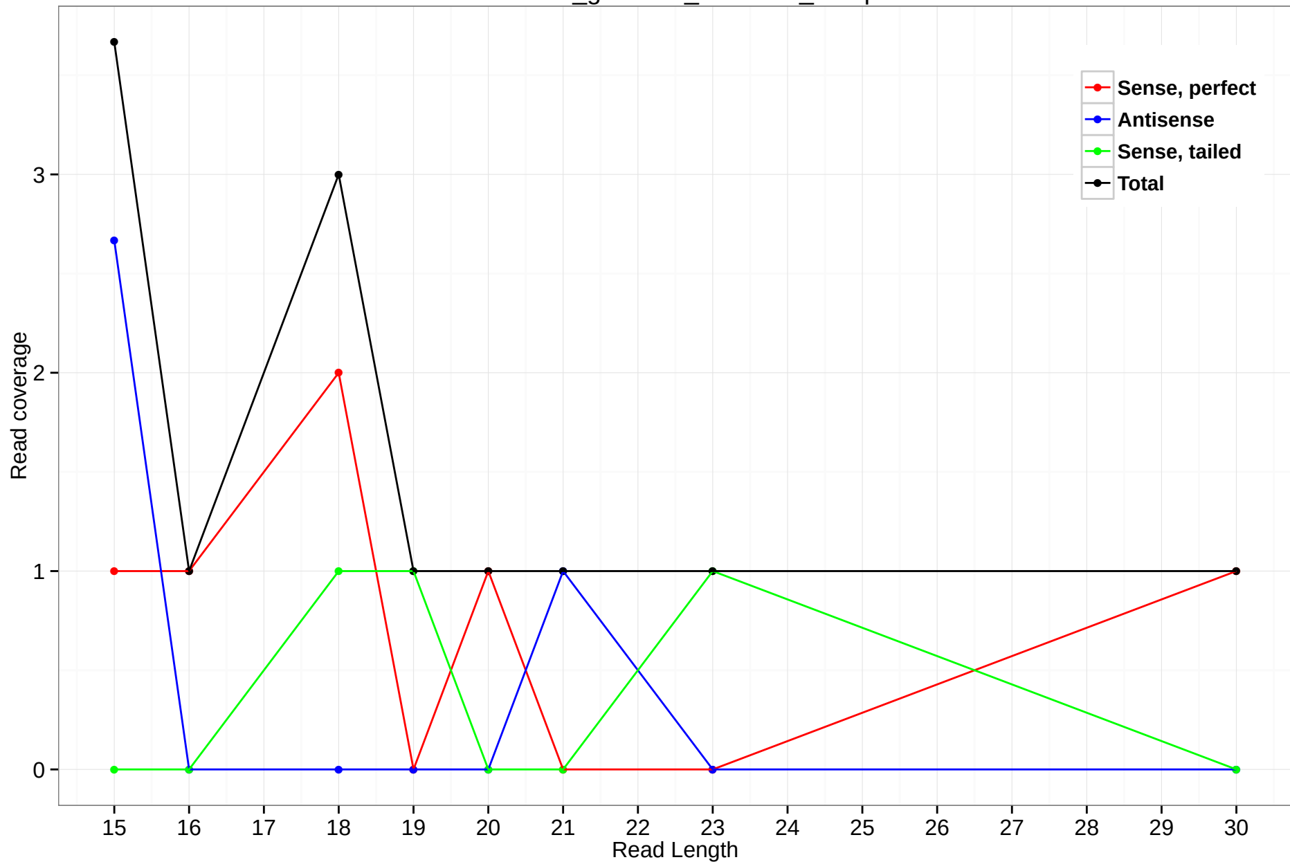
rheMac3_genscan_chr4.934_27.5p
