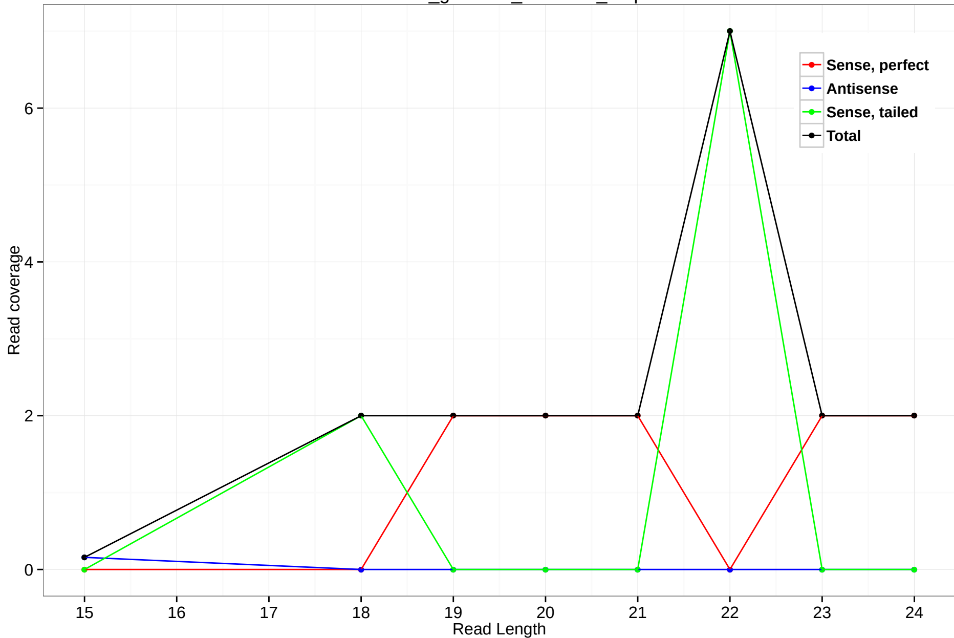
rheMac3_genscan_chr4.910_0.3p
