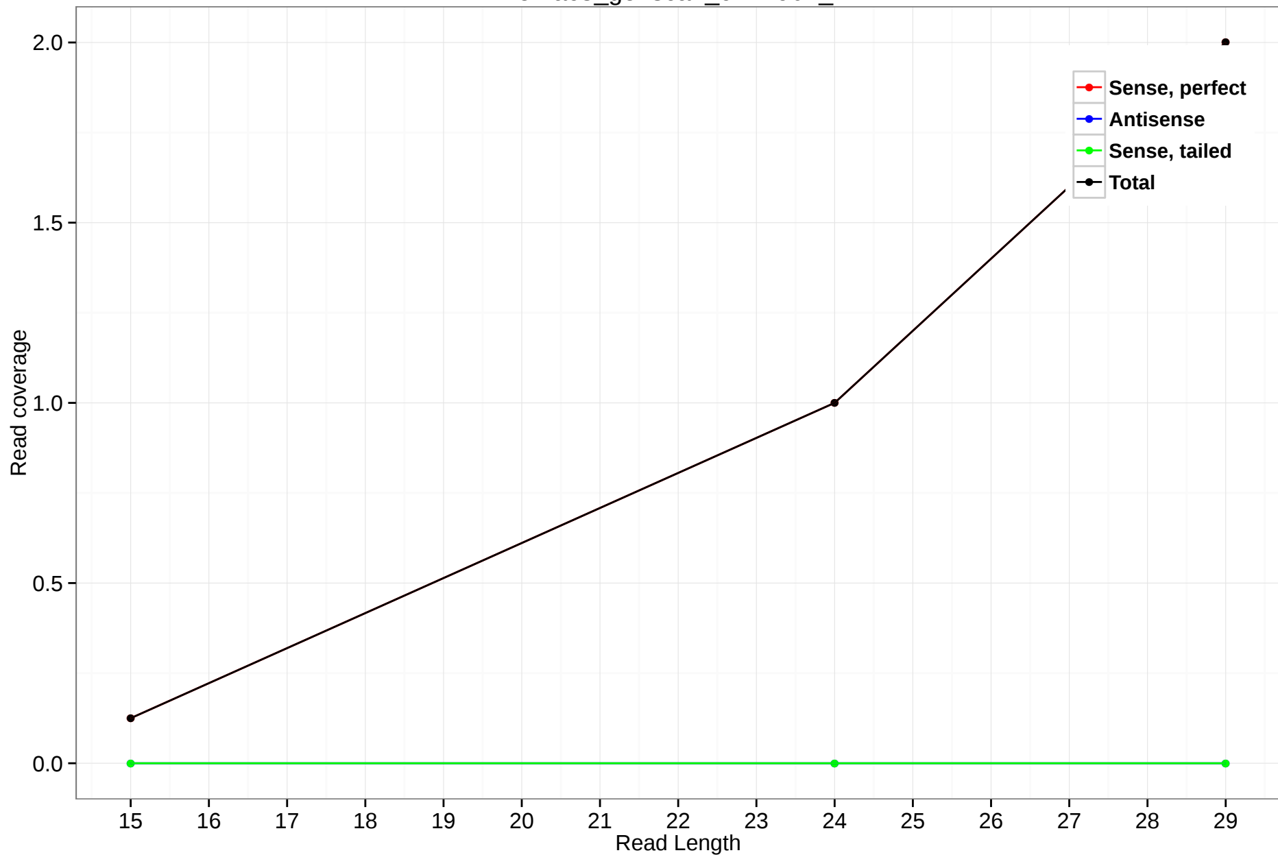
rheMac3_genscan_chr4.902_21
