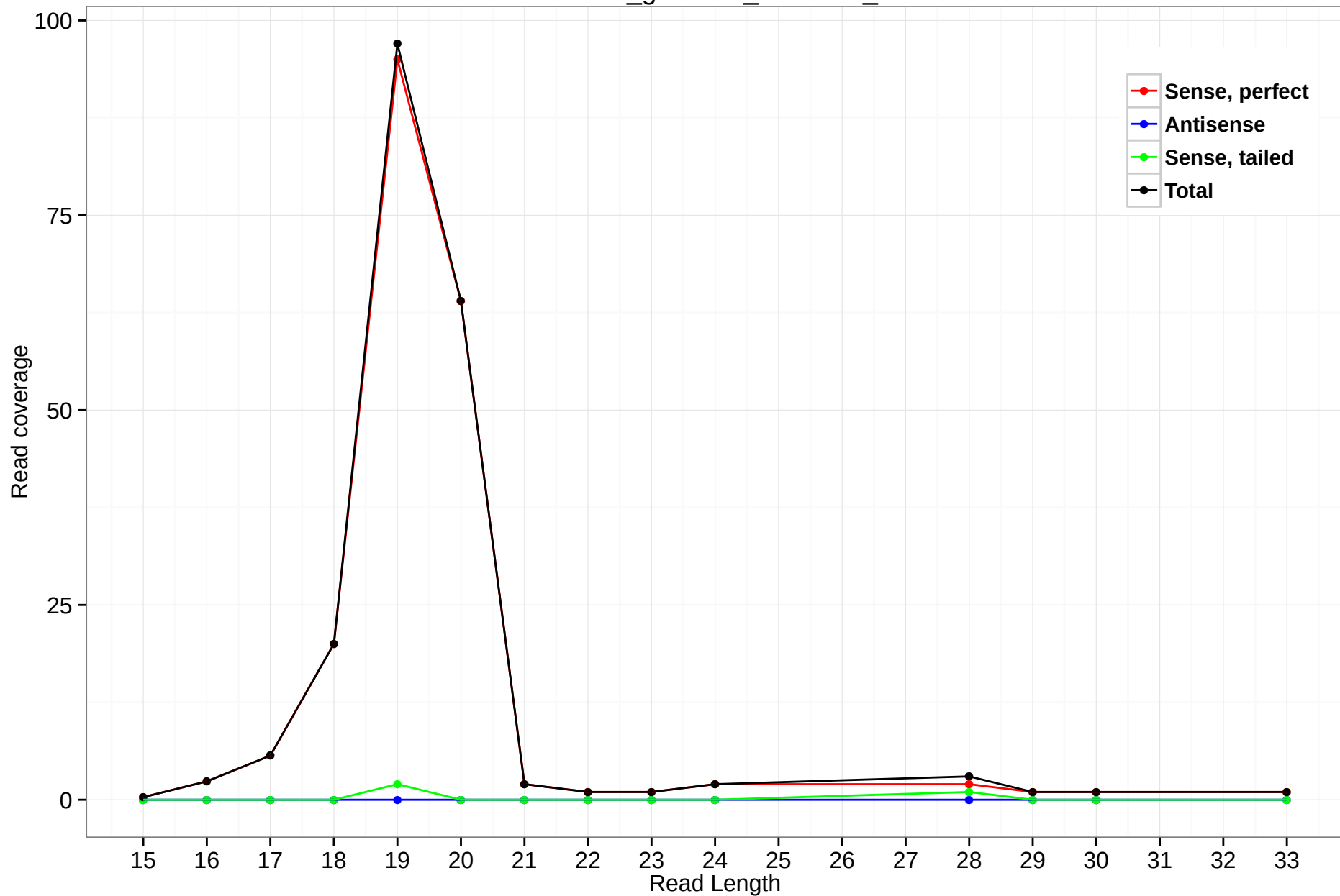
rheMac3_genscan_chr4.902_16
