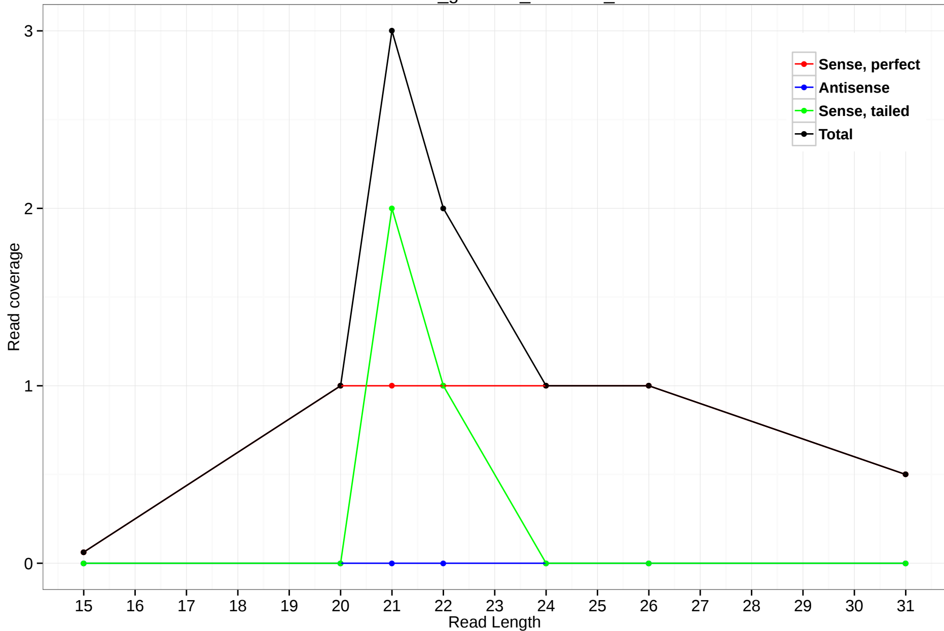
rheMac3_genscan_chr4.901_1
