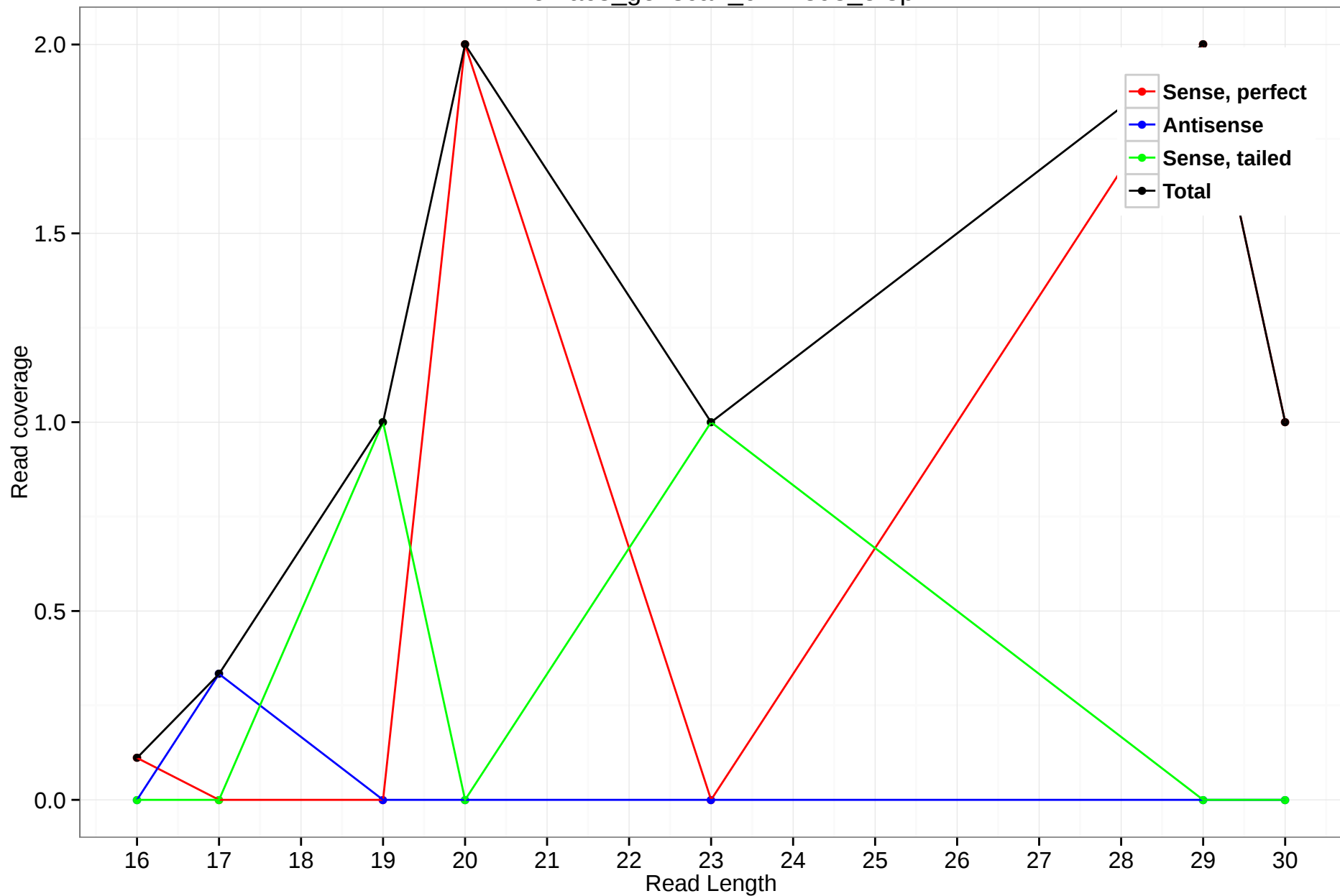
rheMac3_genscan_chr4.898_5.3p
