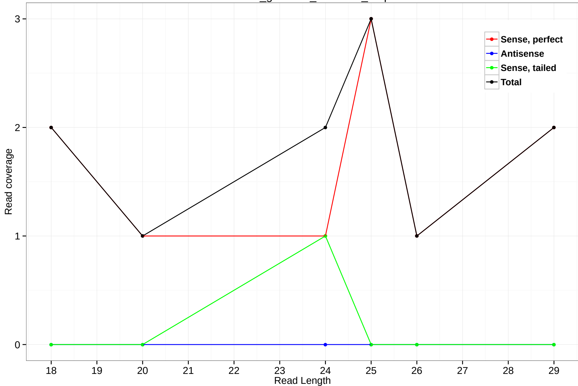
rheMac3_genscan_chr4.876_2.3p
