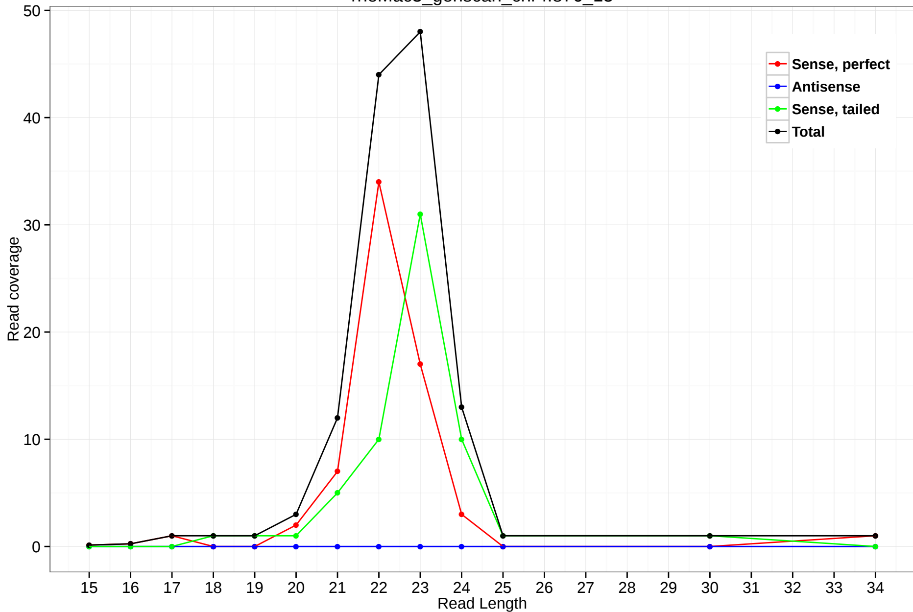
rheMac3_genscan_chr4.876_15
