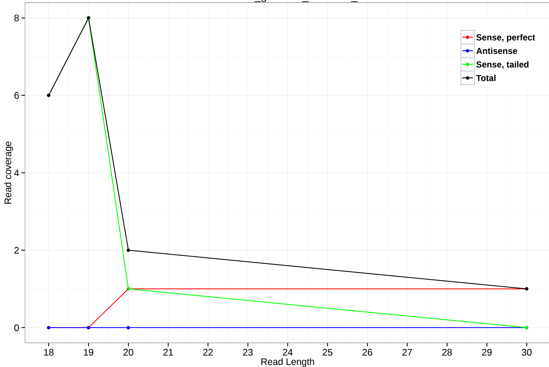
rheMac3_genscan_chr4.871_2
