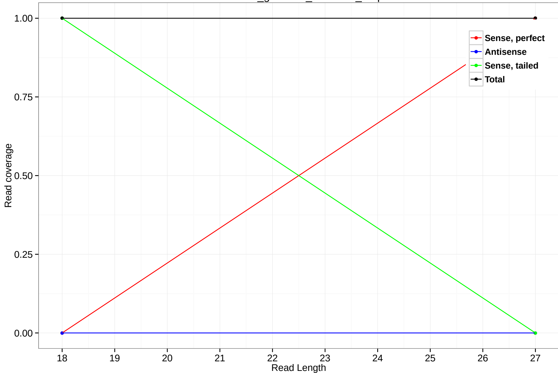
rheMac3_genscan_chr4.870_3.3p
