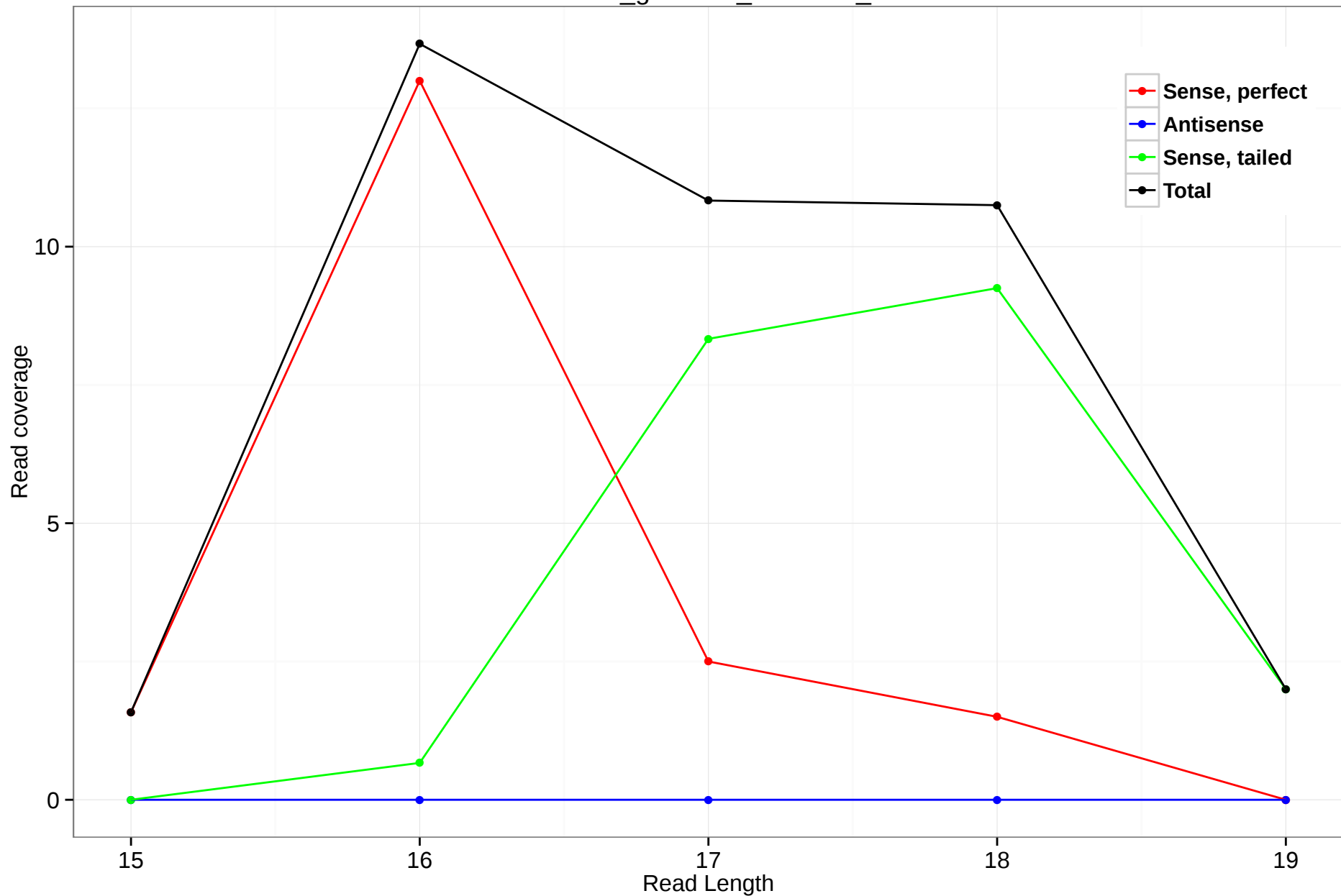
rheMac3_genscan_chr4.858_51
