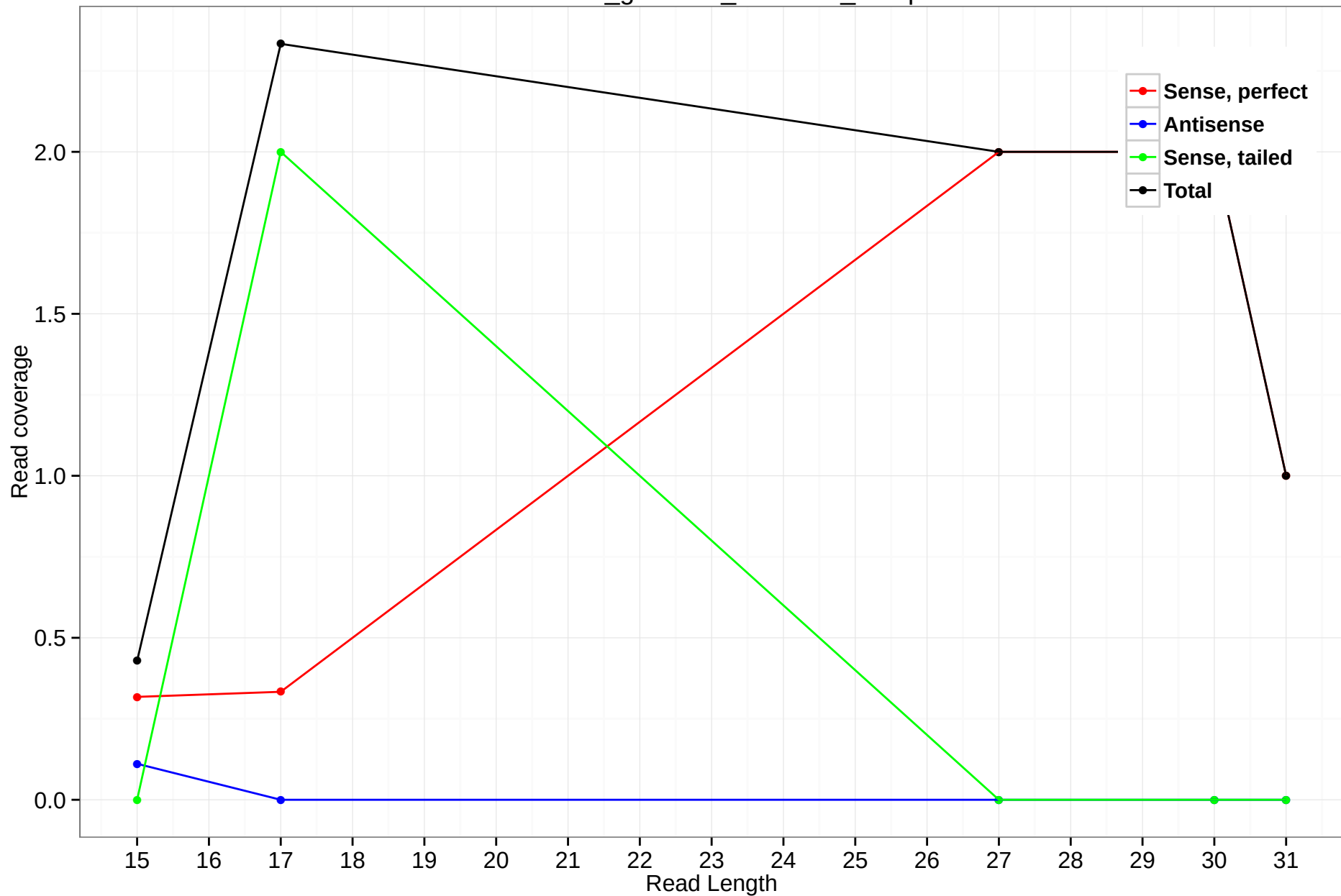
rheMac3_genscan_chr4.858_35.3p
