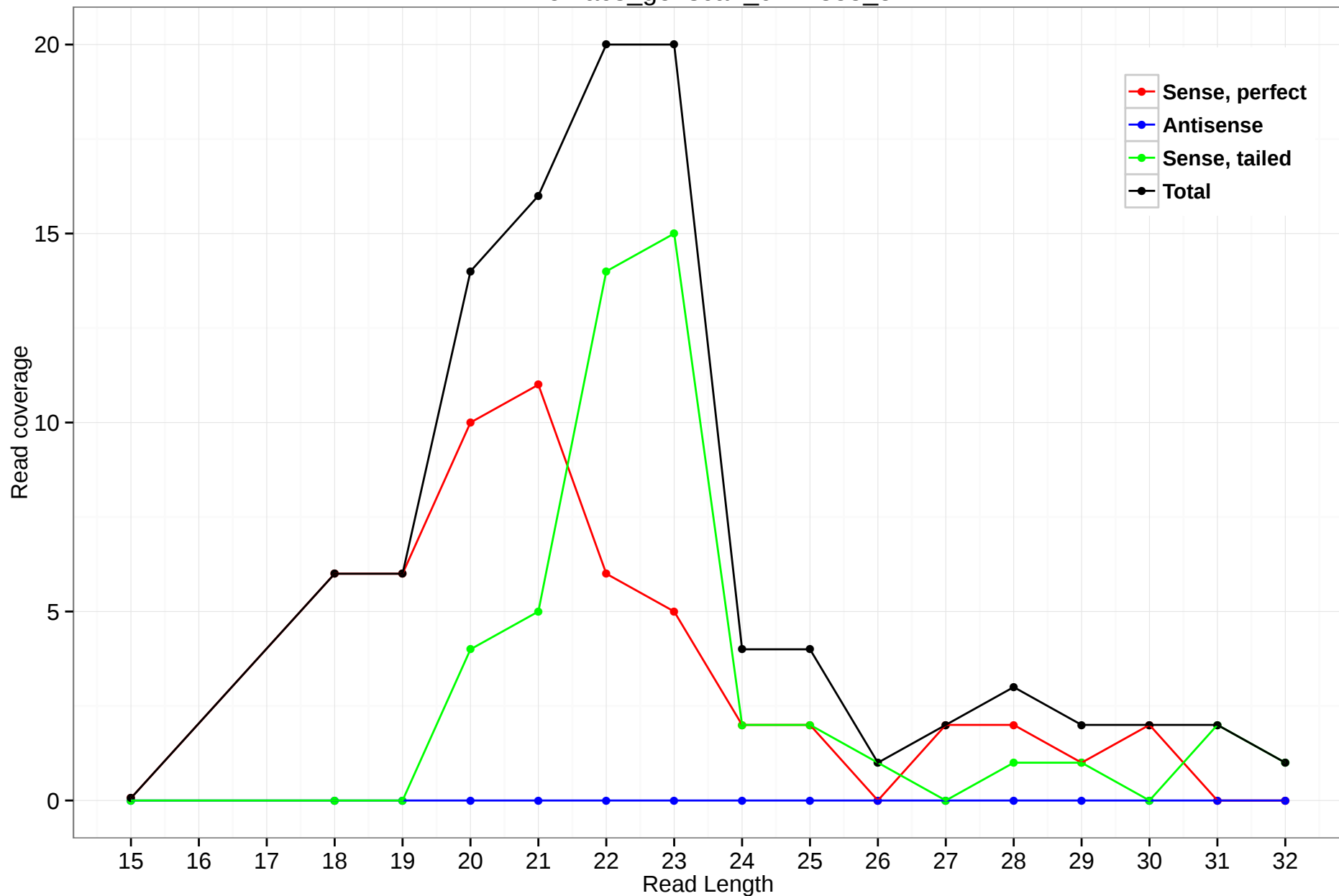
rheMac3_genscan_chr4.855_5
