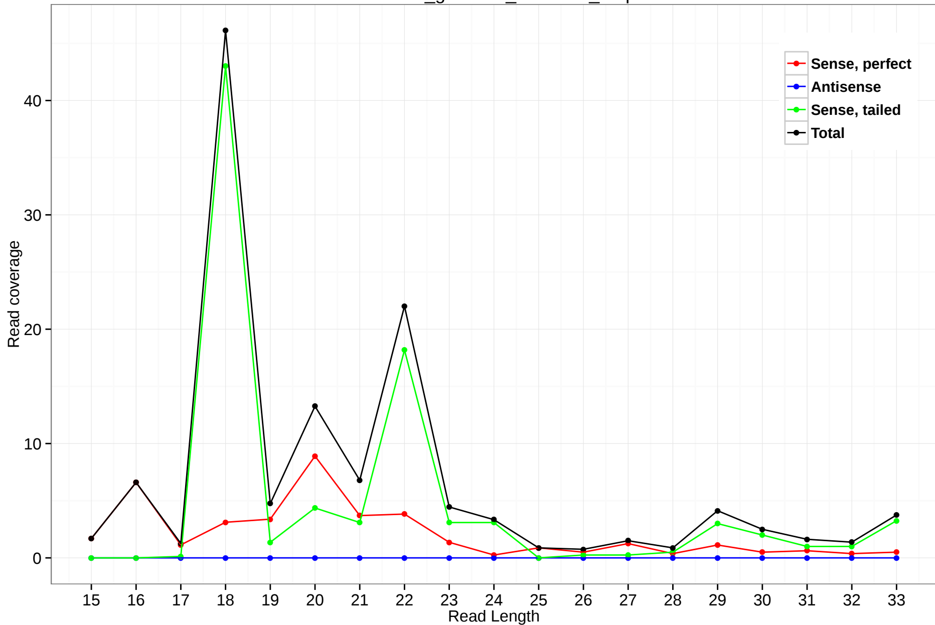
rheMac3_genscan_chr4.756_0.5p
