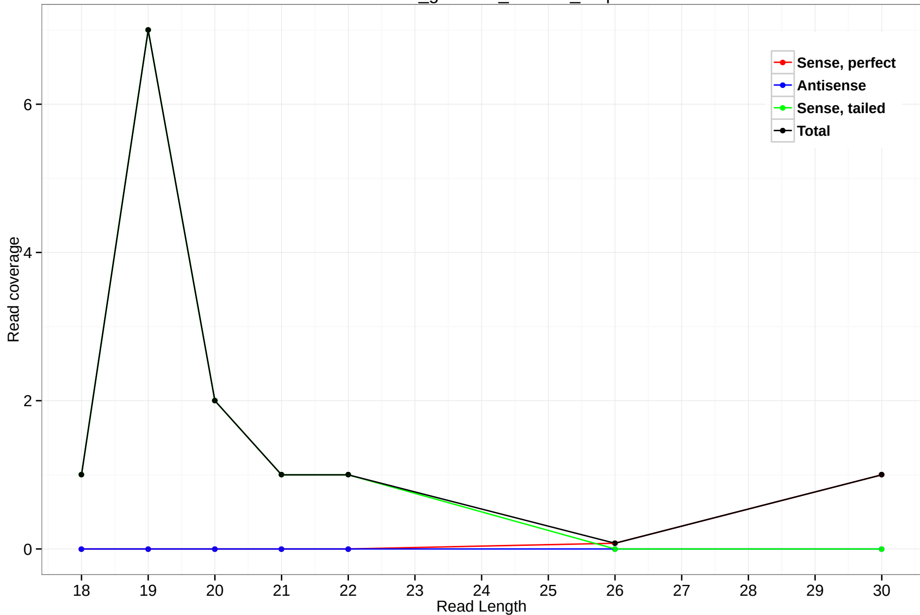
rheMac3_genscan_chr4.67_1.3p
