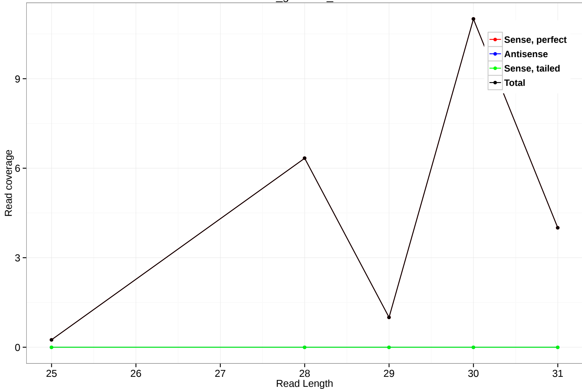
rheMac3_genscan_chr4.676
