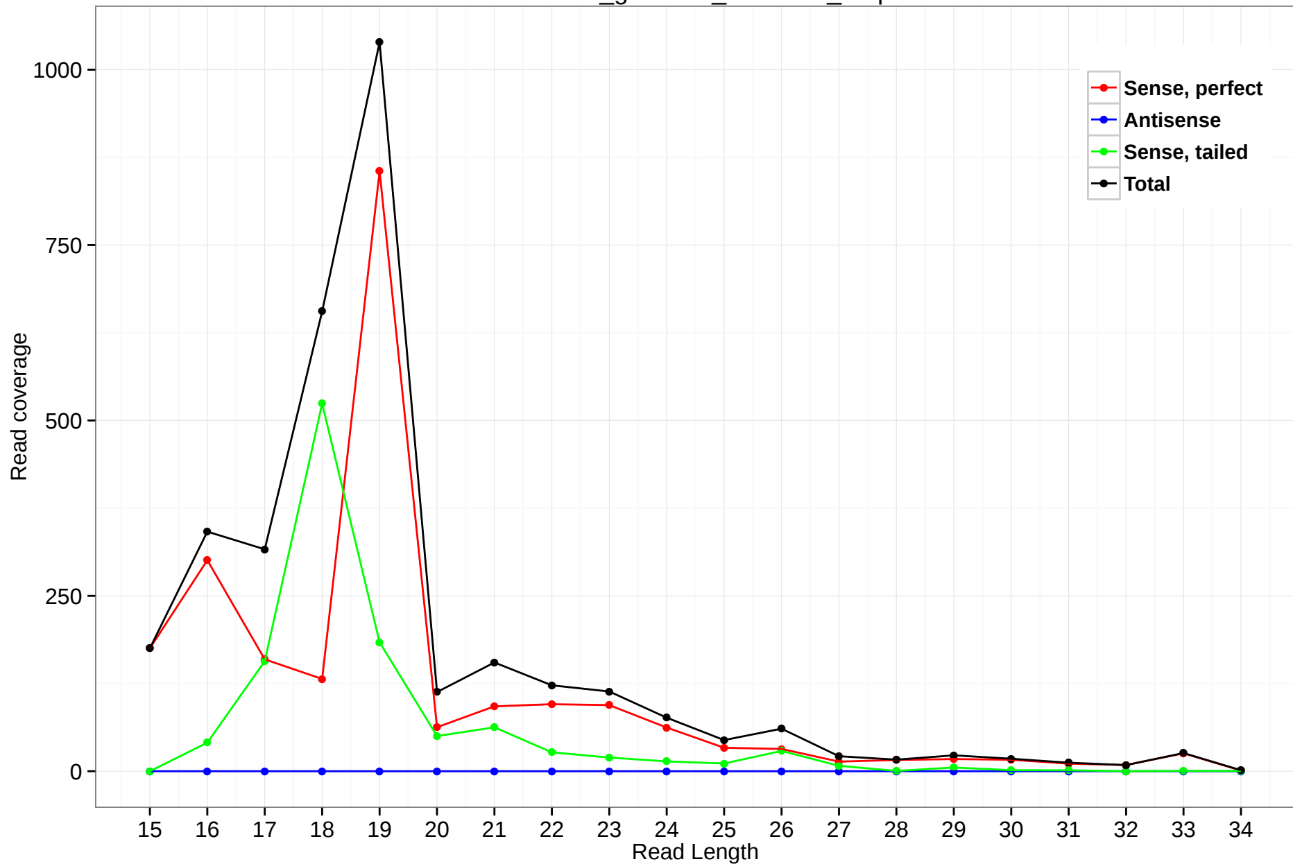
rheMac3_genscan_chr4.661_2.5p
