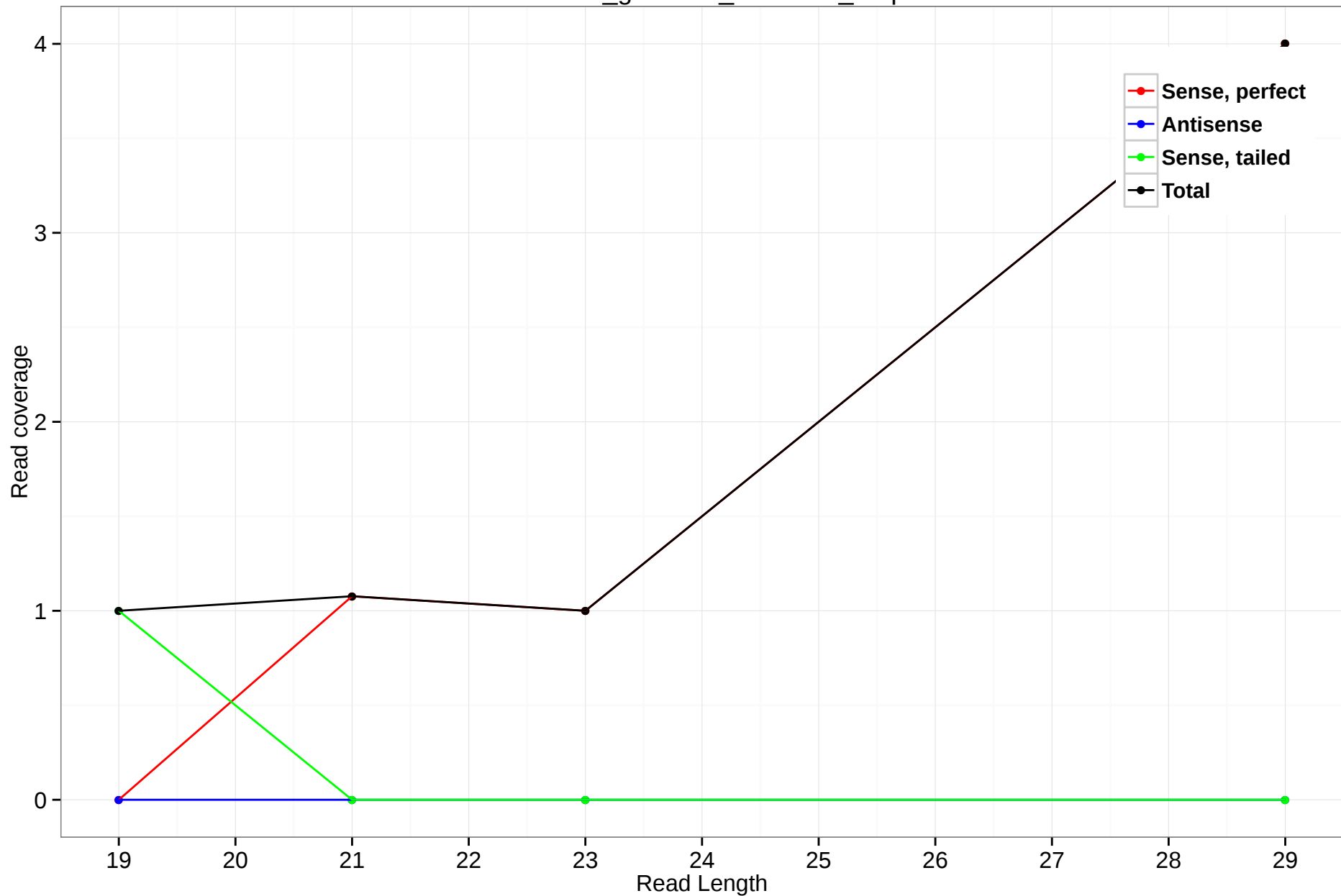
rheMac3_genscan_chr4.640_0.5p
