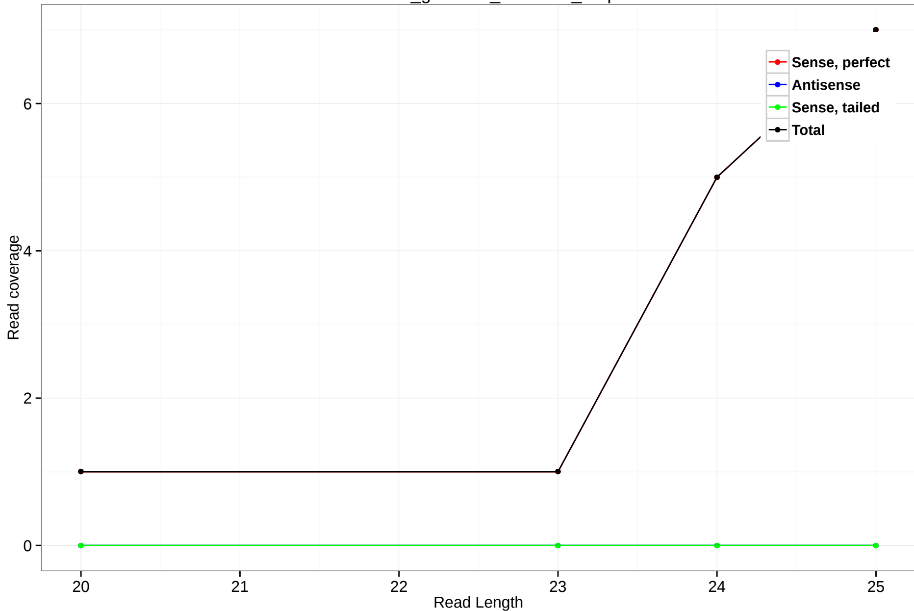
rheMac3_genscan_chr4.603_4.3p
