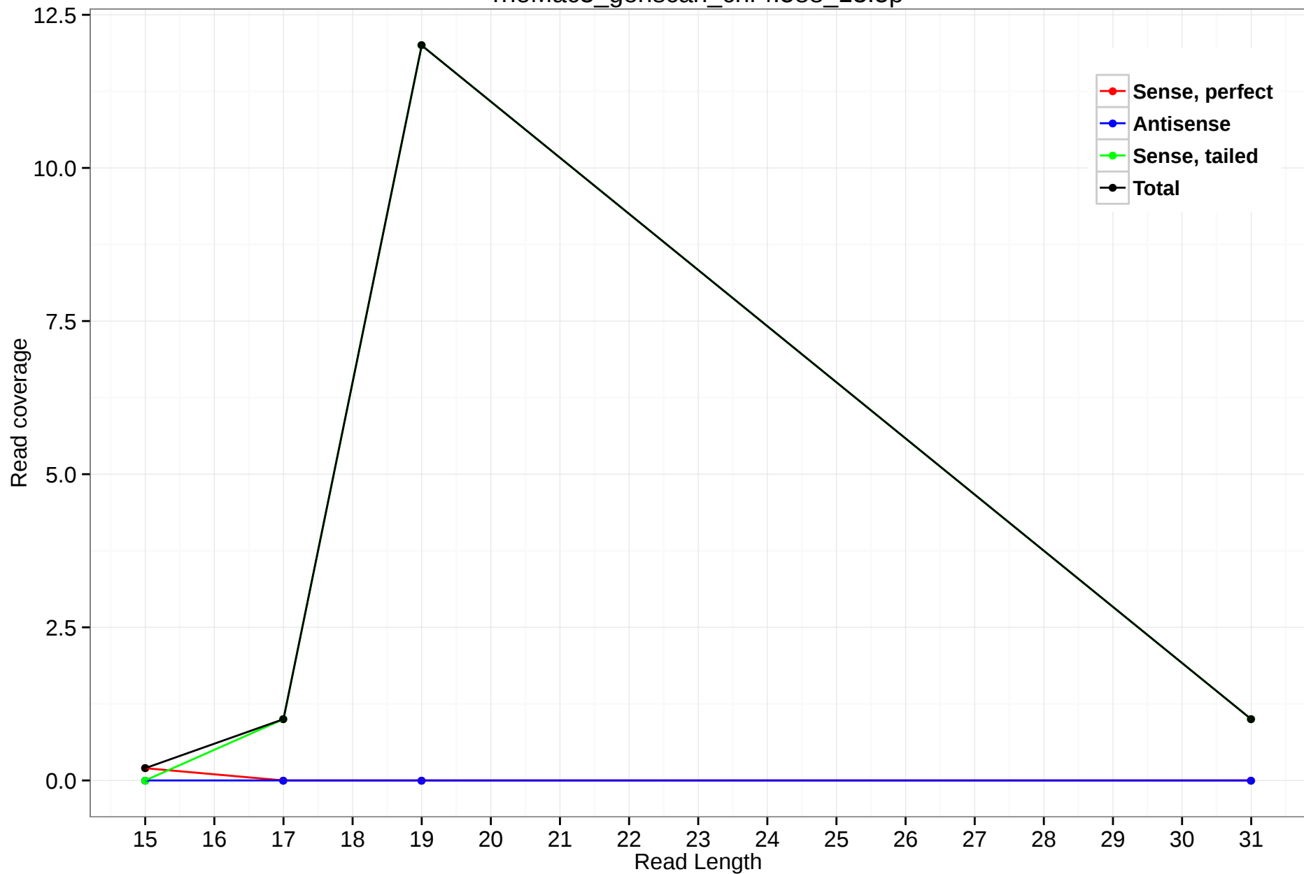
rheMac3_genscan_chr4.588_13.5p
