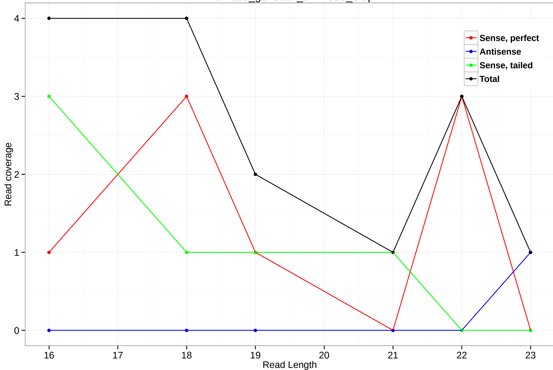
rheMac3_genscan_chr4.586_3.5p
