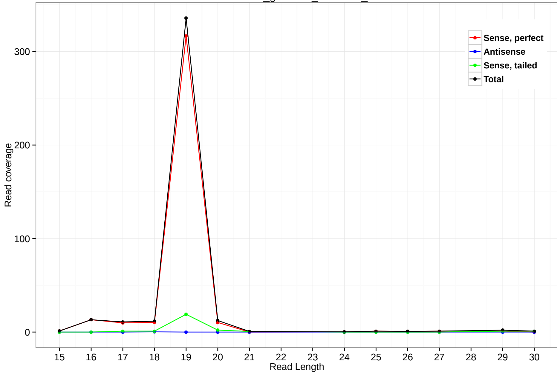
rheMac3_genscan_chr4.488_5
