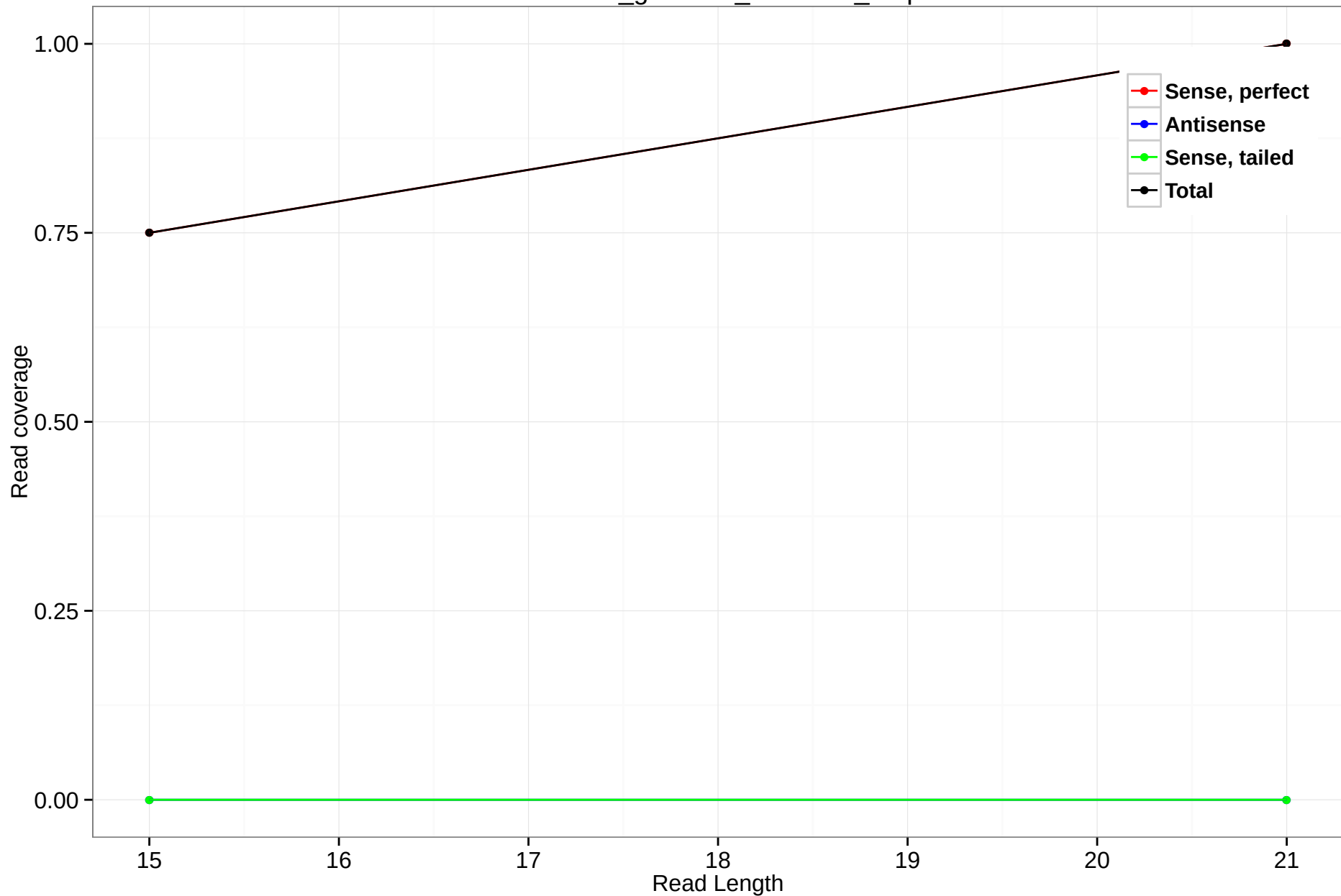
rheMac3_genscan_chr4.465_3.3p
