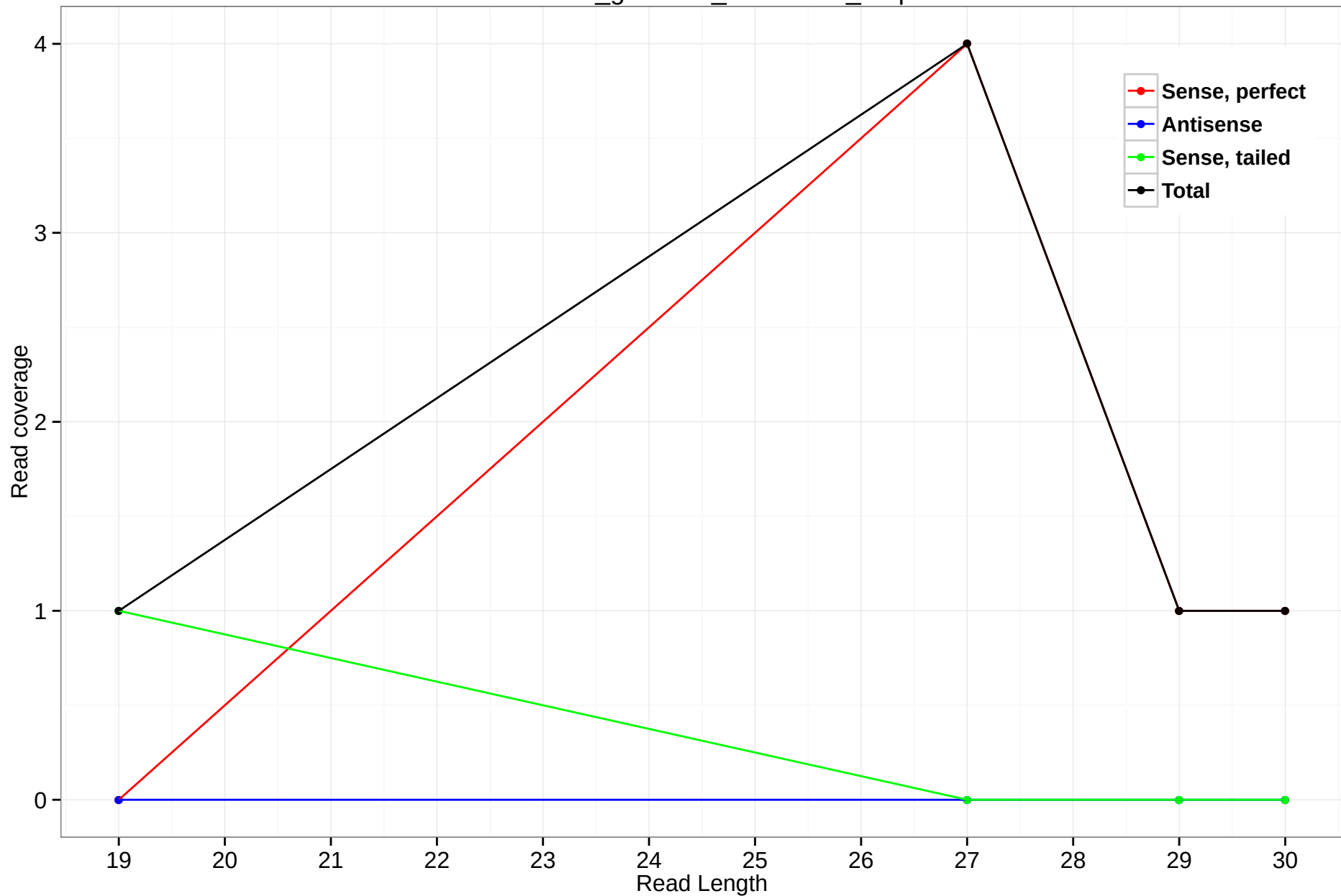
rheMac3_genscan_chr4.3445_2.3p
