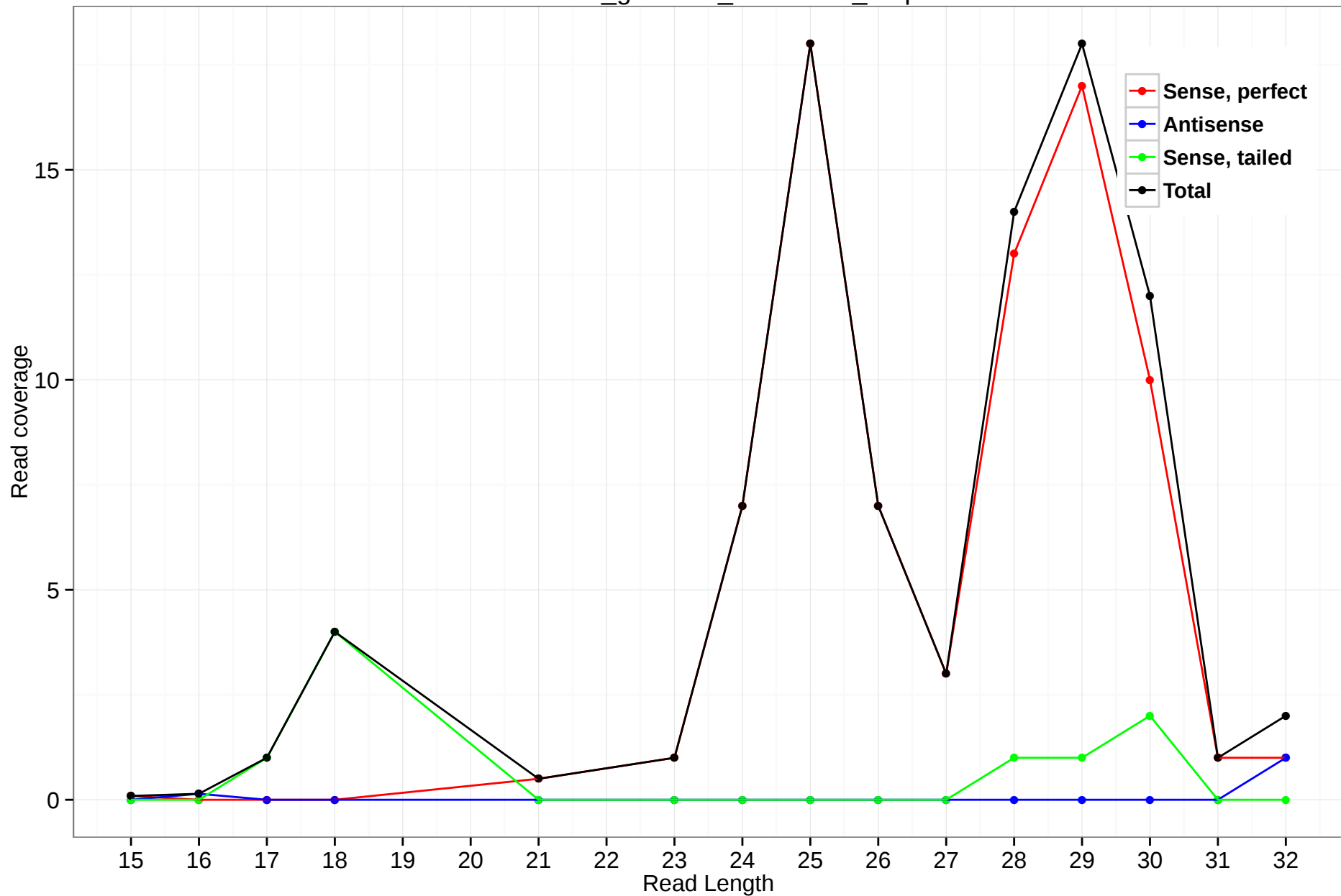
rheMac3_genscan_chr4.3445_1.5p
