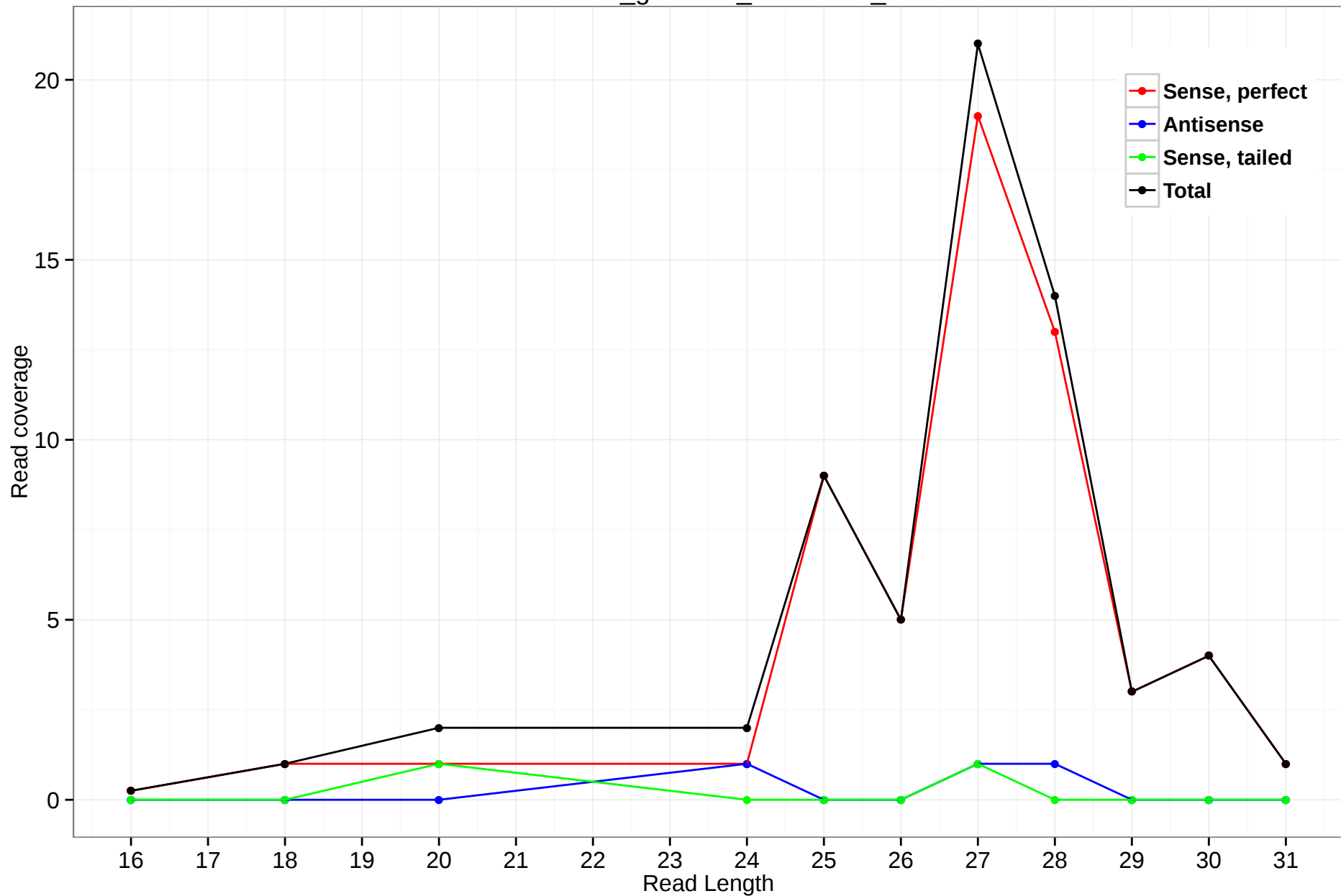
rheMac3_genscan_chr4.3445_0
