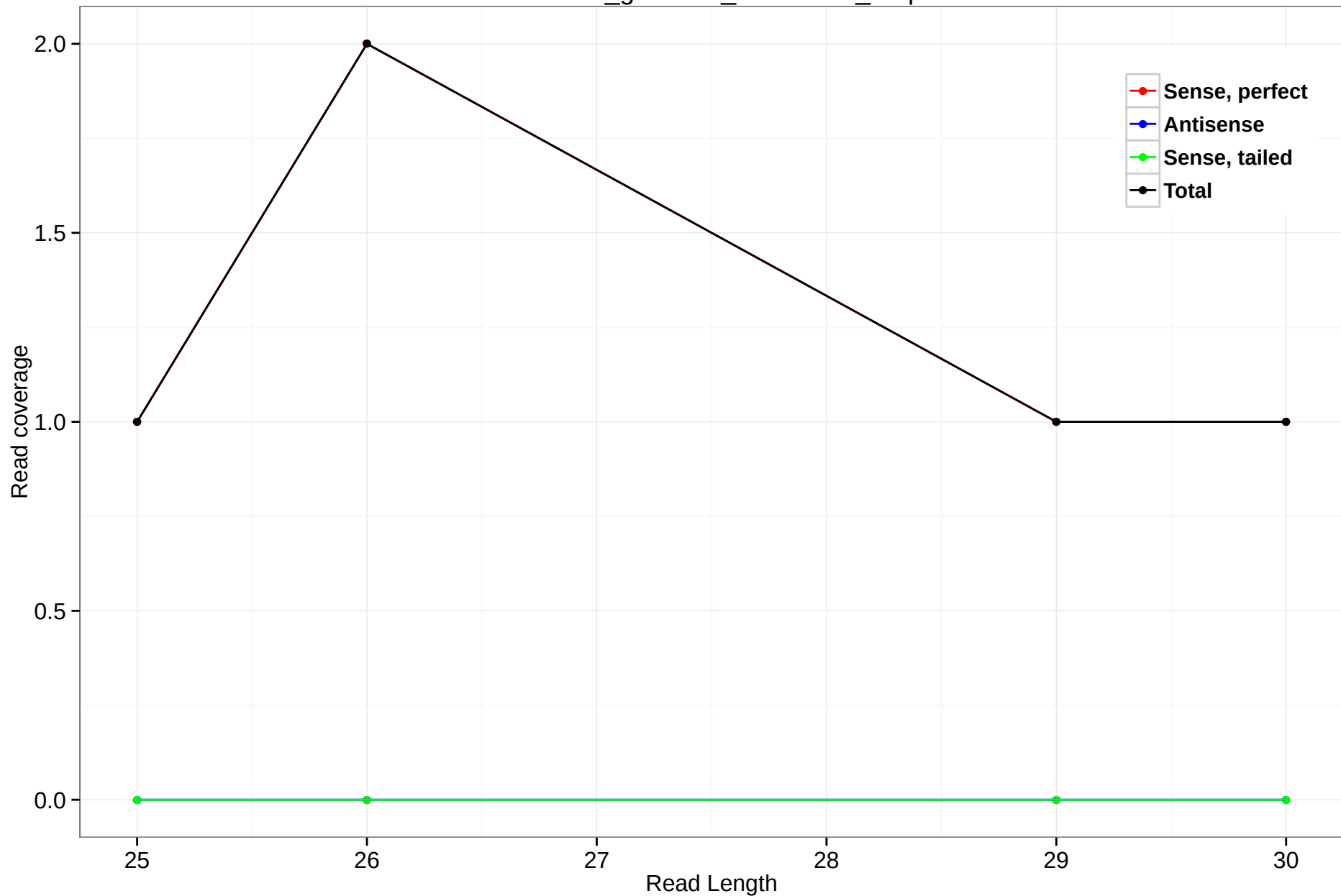
rheMac3_genscan_chr4.3442_0.3p
