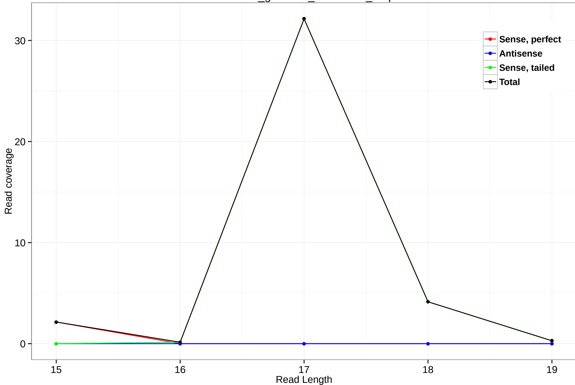
rheMac3_genscan_chr4.3340_1.3p
