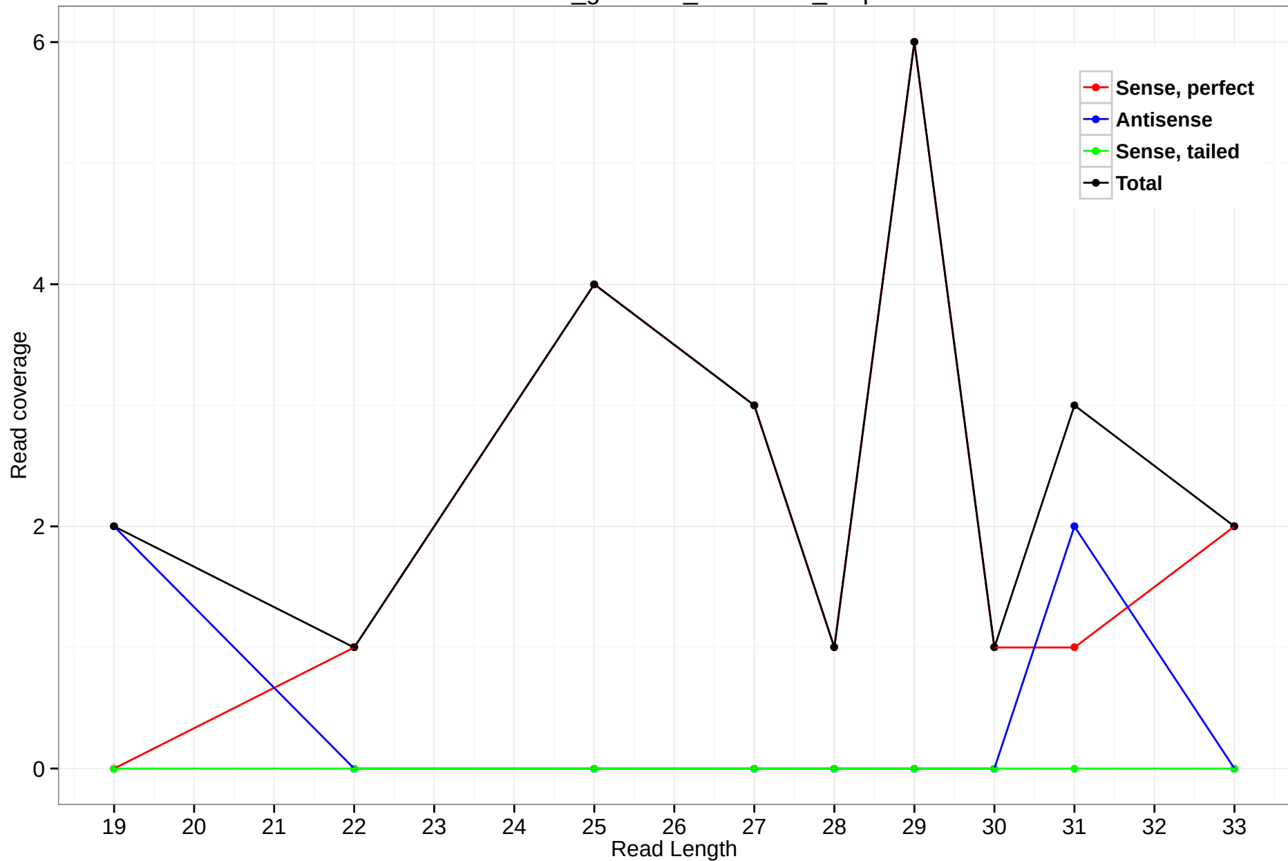
rheMac3_genscan_chr4.3260_7.5p
