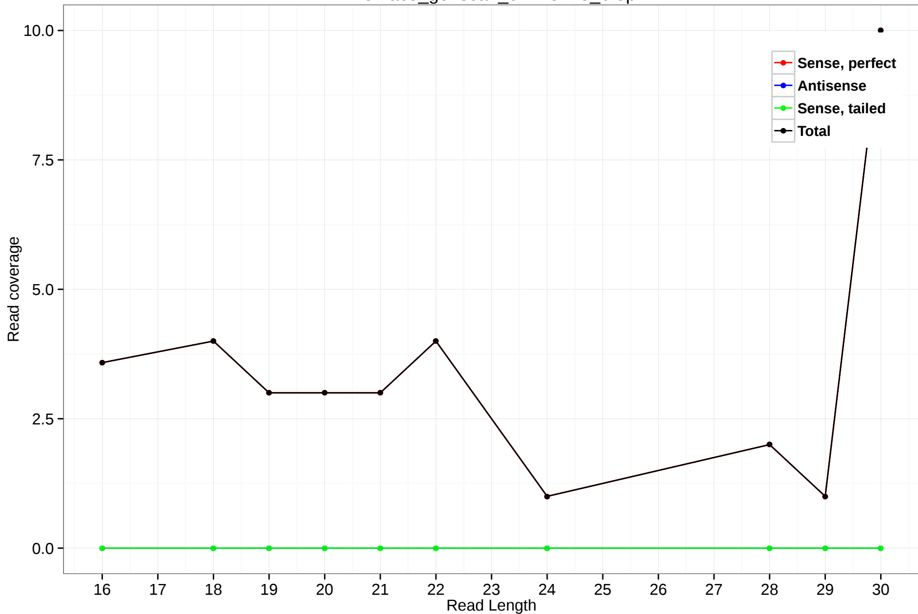
rheMac3_genscan_chr4.3245_6.5p
