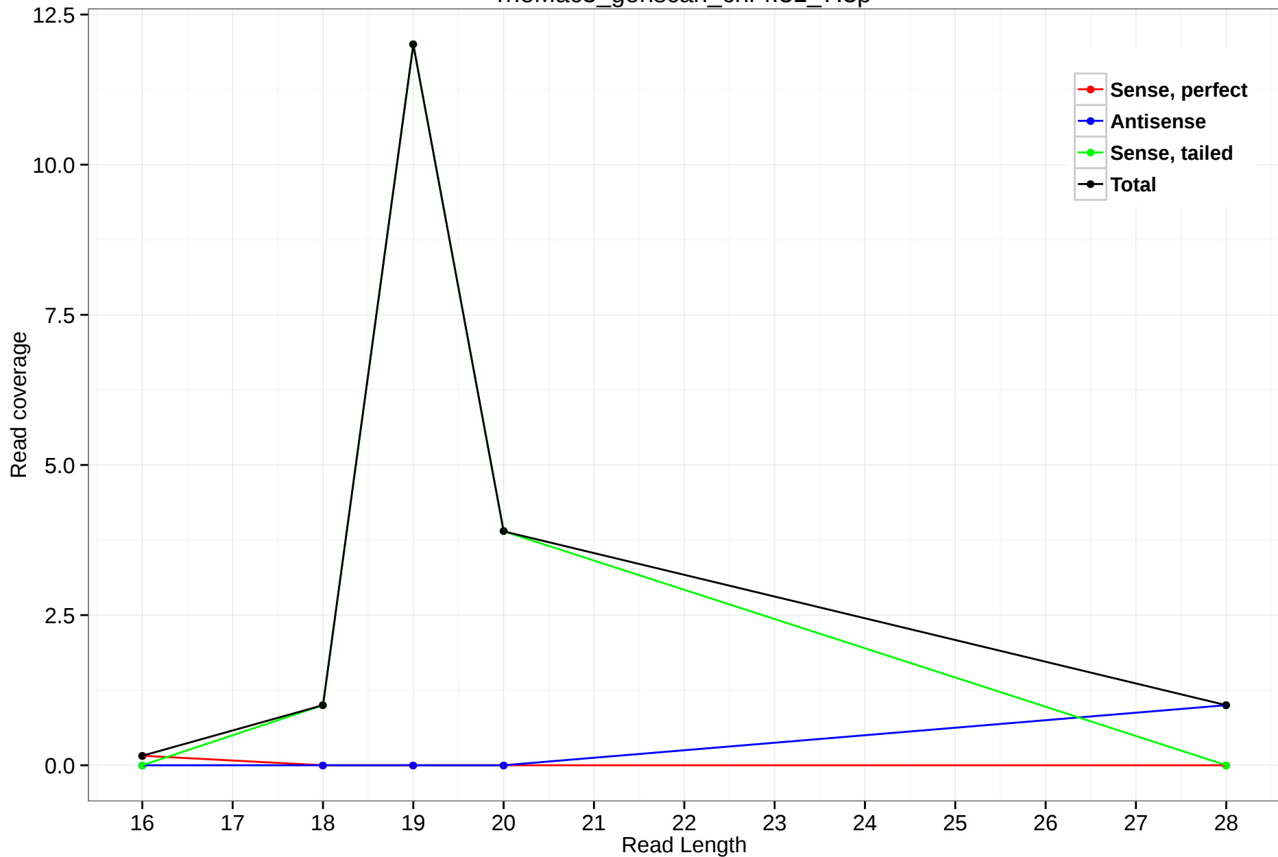
rheMac3_genscan_chr4.31_7.3p
