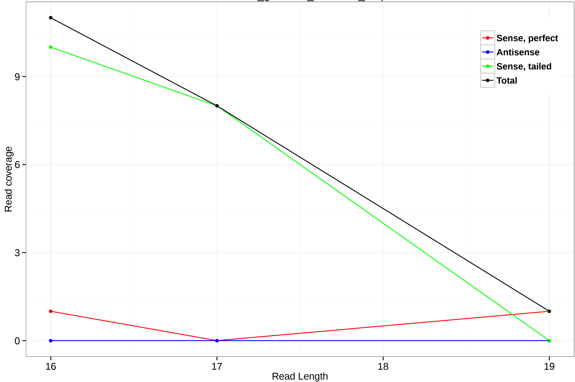
rheMac3_genscan_chr4.319_2.5p
