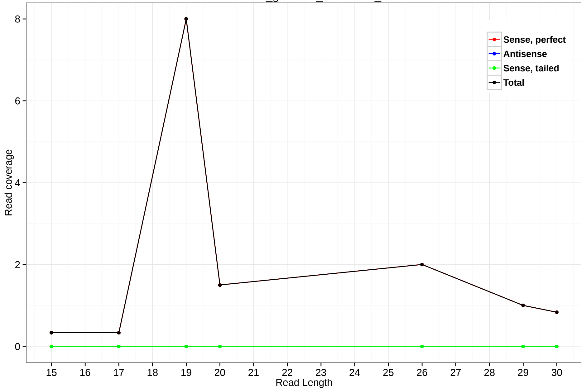
rheMac3_genscan_chr4.3147_6
