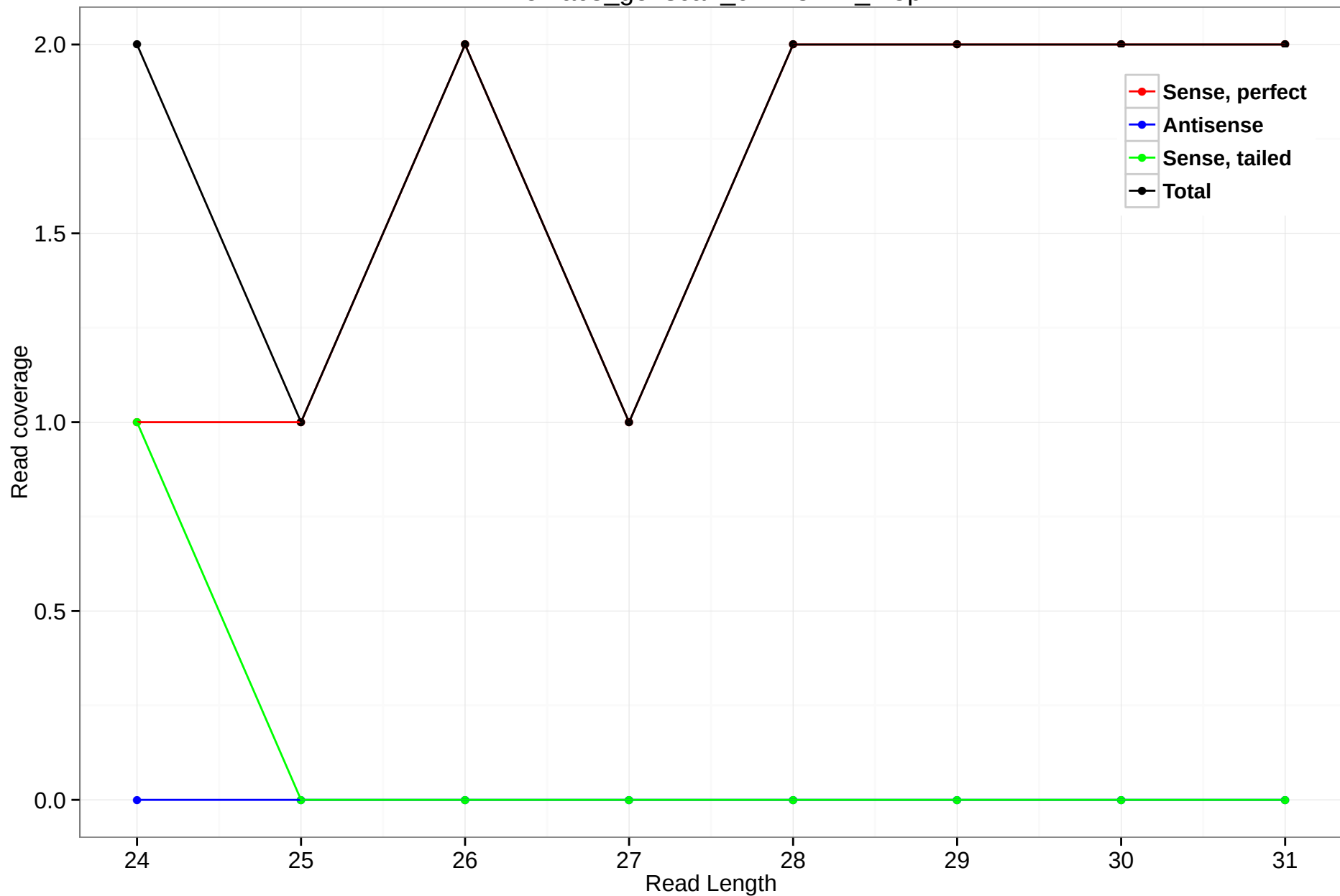
rheMac3_genscan_chr4.3122_4.5p
