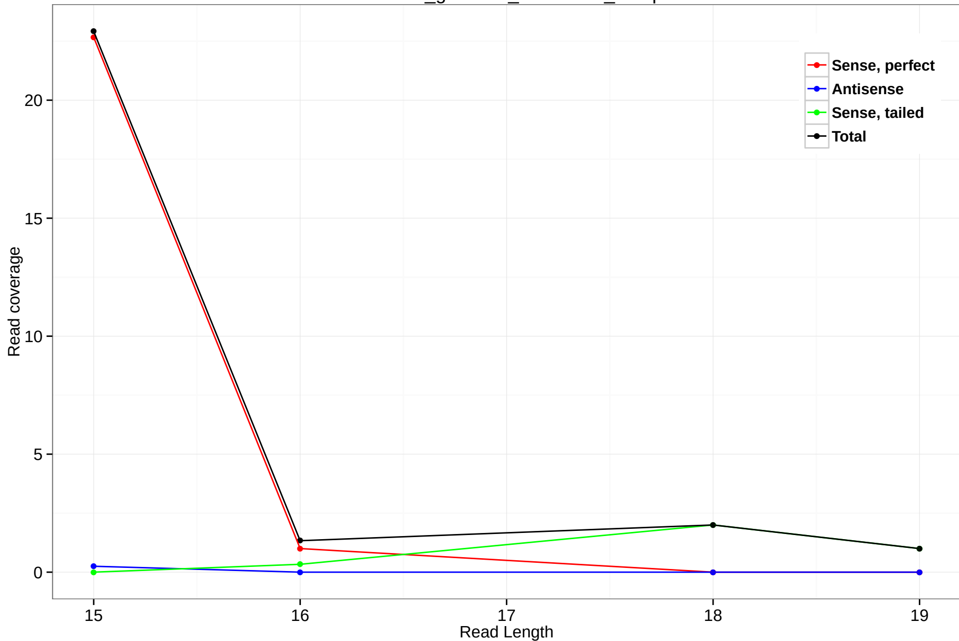
rheMac3_genscan_chr4.3080_21.5p
