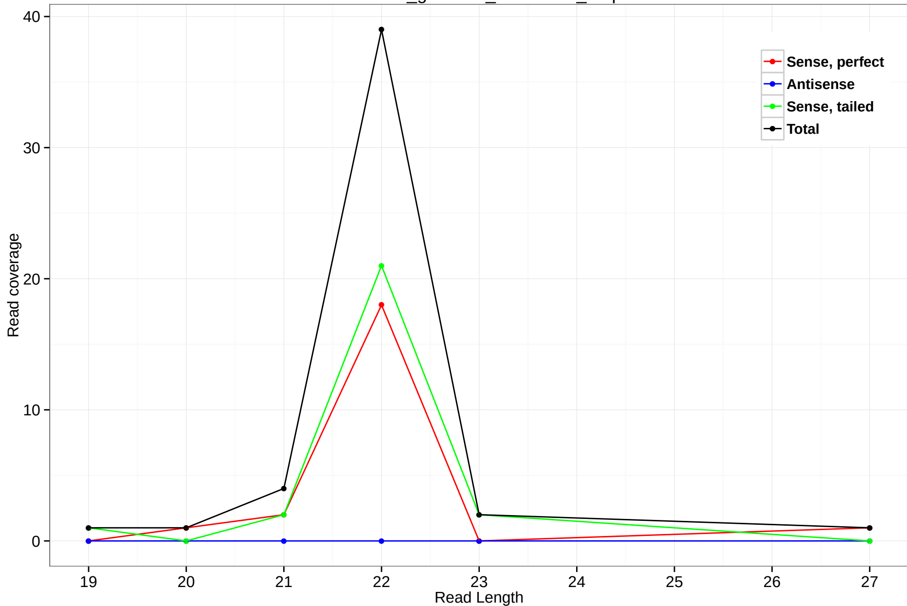
rheMac3_genscan_chr4.3025_9.3p
