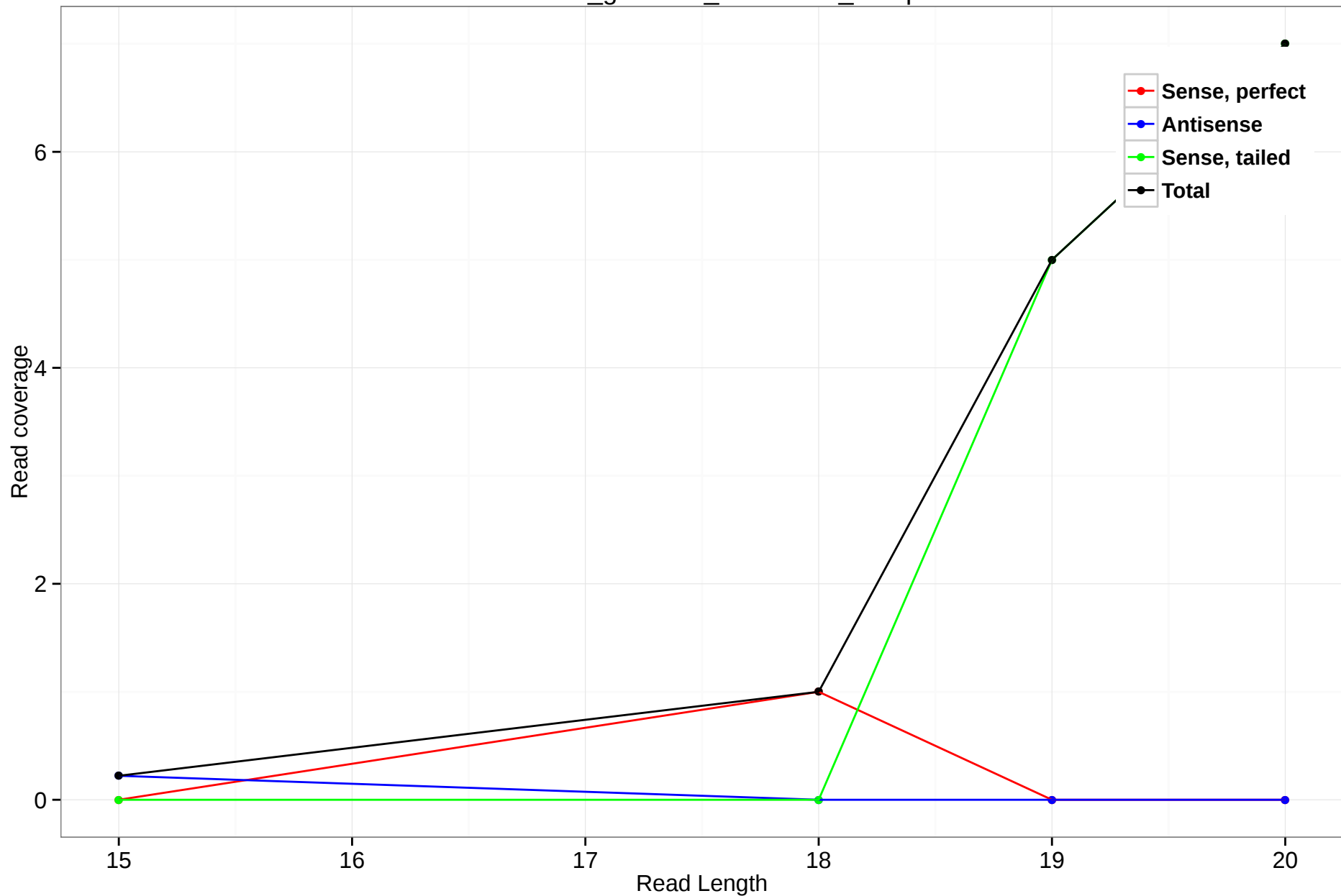
rheMac3_genscan_chr4.3025_13.3p
